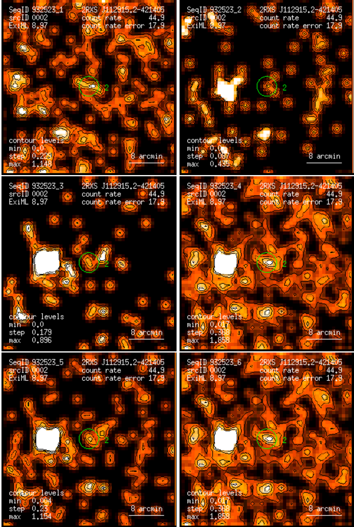
Figure 2: RASS 932523: detection 0002: band rate images, Gaussian filter: (1) PSPC channels 11 – 41, (2) 52 – 90, (3) 91 – 201, (4) 11 – 235, (5) 52 – 201, (6) 11 – 201. Broad band rates in counts/ks. Band rate contour levels in counts/ks/arcmin 2 .
