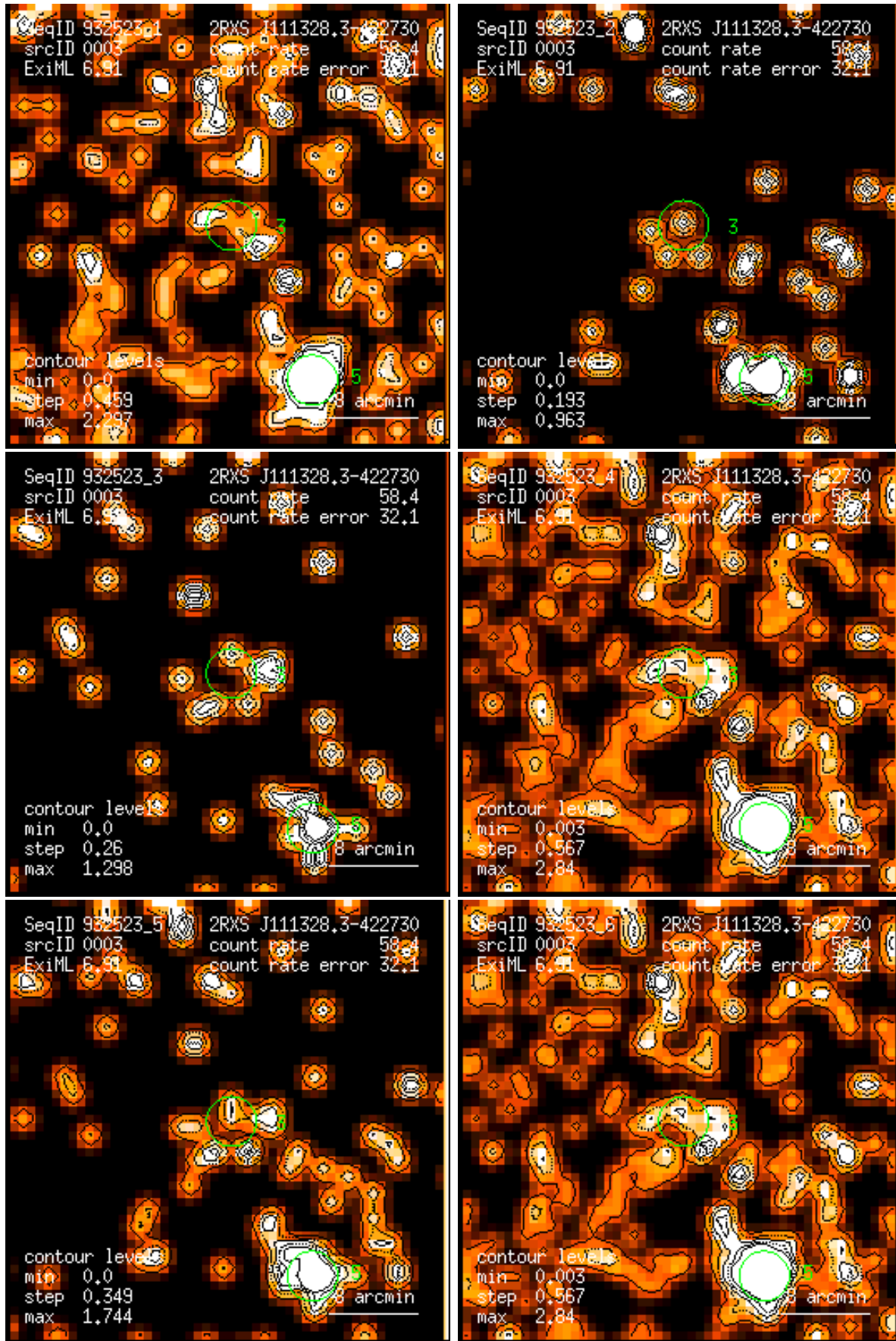
Figure 3: RASS 932523: detection 0003: band rate images, Gaussian filter: (1) PSPC channels 11 – 41, (2) 52 – 90, (3) 91 – 201, (4) 11 – 235, (5) 52 – 201, (6) 11 – 201. Broad band rates in counts/ks. Band rate contour levels in counts/ks/arcmin 2 .
