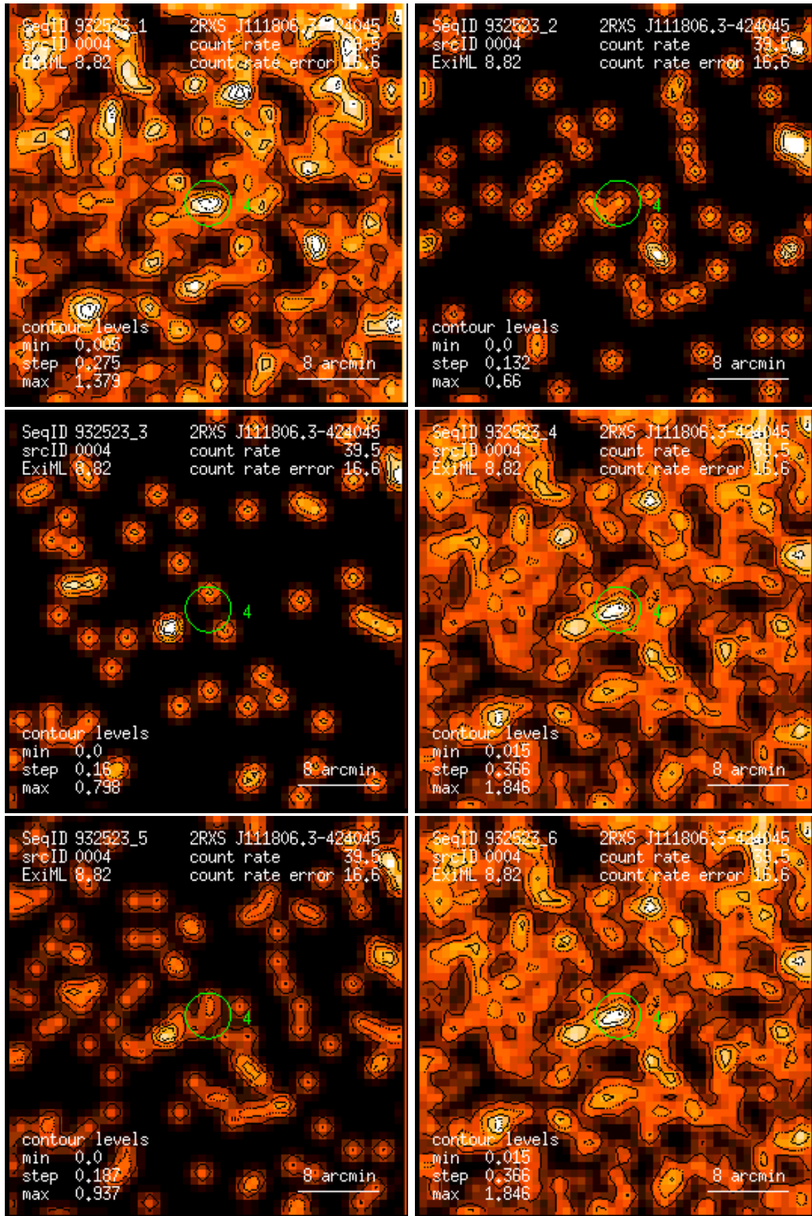
Figure 4: RASS 932523: detection 0004: band rate images, Gaussian filter: (1) PSPC channels 11 – 41, (2) 52 – 90, (3) 91 – 201, (4) 11 – 235, (5) 52 – 201, (6) 11 – 201. Broad band rates in counts/ks. Band rate contour levels in counts/ks/arcmin 2 .
