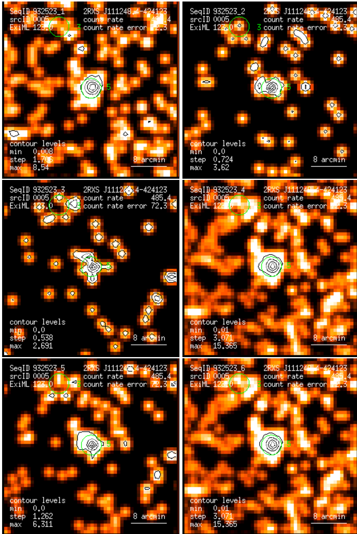
Figure 5: RASS 932523: detection 0005: band rate images, Gaussian filter: (1) PSPC channels 11 – 41, (2) 52 – 90, (3) 91 – 201, (4) 11 – 235, (5) 52 – 201, (6) 11 – 201. Broad band rates in counts/ks. Band rate contour levels in counts/ks/arcmin 2 .
