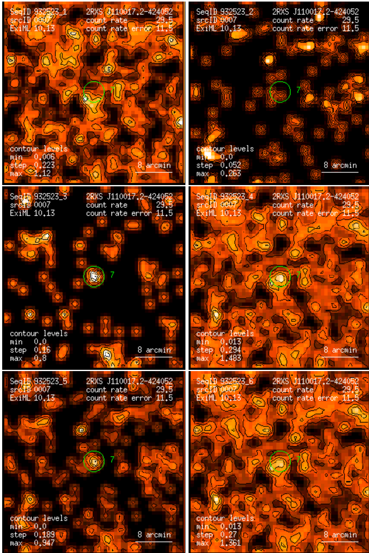
Figure 7: RASS 932523: detection 0007: band rate images, Gaussian filter: (1) PSPC channels 11 – 41, (2) 52 – 90, (3) 91 – 201, (4) 11 – 235, (5) 52 – 201, (6) 11 – 201. Broad band rates in counts/ks. Band rate contour levels in counts/ks/arcmin 2 .
