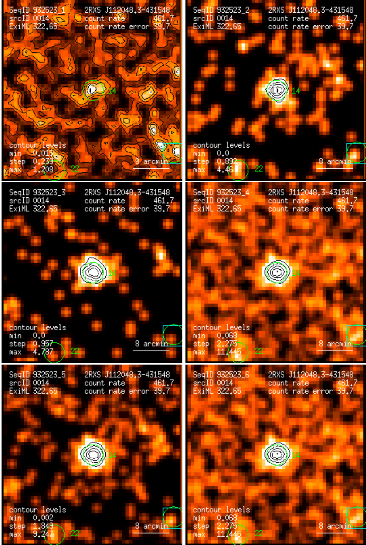
Figure 14: RASS 932523: detection 0014: band rate images, Gaussian filter: (1) PSPC channels 11 – 41, (2) 52 – 90, (3) 91 – 201, (4) 11 – 235, (5) 52 – 201, (6) 11 – 201. Broad band rates in counts/ks. Band rate contour levels in counts/ks/arcmin 2 .
