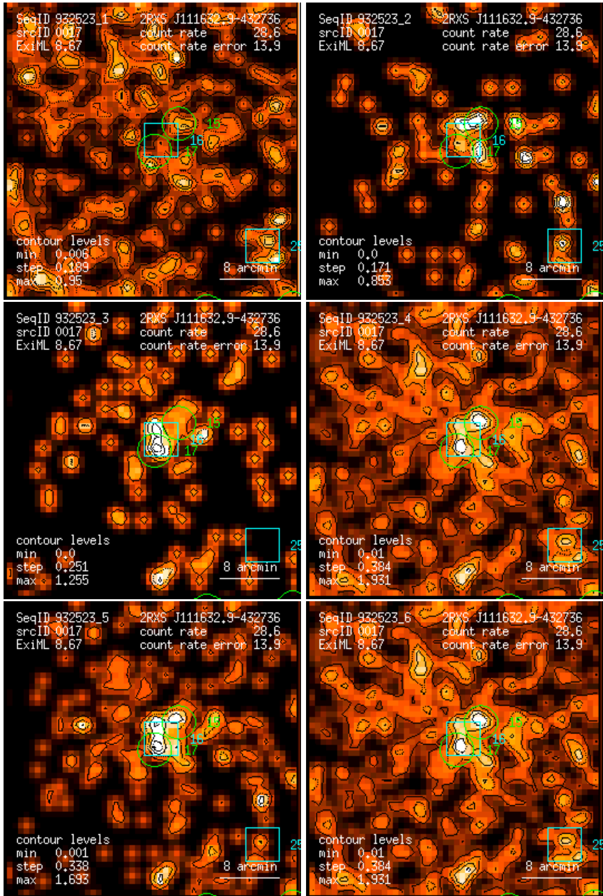
Figure 17: RASS 932523: detection 0017: band rate images, Gaussian filter: (1) PSPC channels 11 – 41, (2) 52 – 90, (3) 91 – 201, (4) 11 – 235, (5) 52 – 201, (6) 11 – 201. Broad band rates in counts/ks. Band rate contour levels in counts/ks/arcmin 2 .
