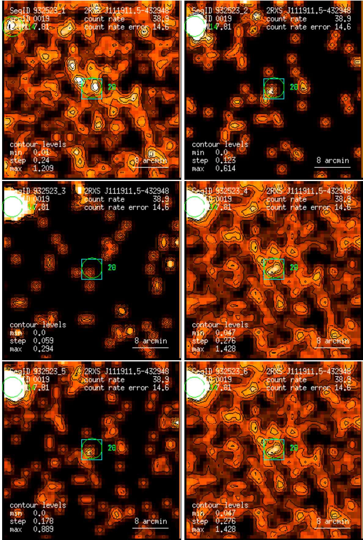
Figure 19: RASS 932523: detection 0019: band rate images, Gaussian filter: (1) PSPC channels 11 – 41, (2) 52 – 90, (3) 91 – 201, (4) 11 – 235, (5) 52 – 201, (6) 11 – 201. Broad band rates in counts/ks. Band rate contour levels in counts/ks/arcmin 2 .
