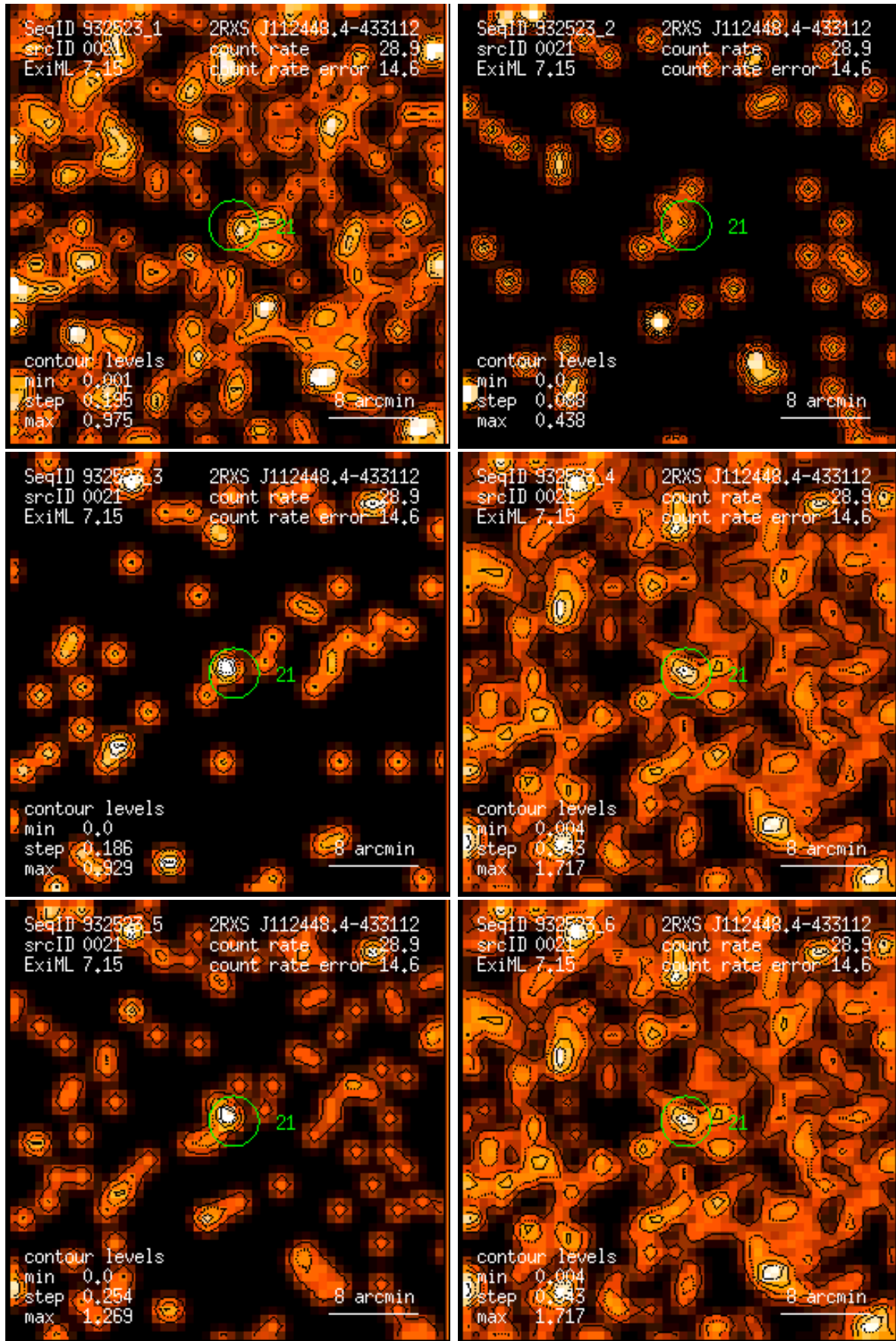
Figure 21: RASS 932523: detection 0021: band rate images, Gaussian filter: (1) PSPC channels 11 – 41, (2) 52 – 90, (3) 91 – 201, (4) 11 – 235, (5) 52 – 201, (6) 11 – 201. Broad band rates in counts/ks. Band rate contour levels in counts/ks/arcmin 2 .
