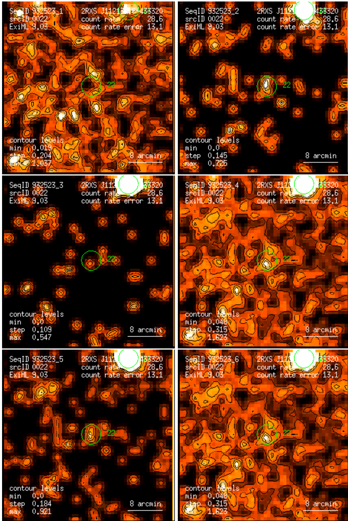
Figure 22: RASS 932523: detection 0022: band rate images, Gaussian filter: (1) PSPC channels 11 – 41, (2) 52 – 90, (3) 91 – 201, (4) 11 – 235, (5) 52 – 201, (6) 11 – 201. Broad band rates in counts/ks. Band rate contour levels in counts/ks/arcmin 2 .
