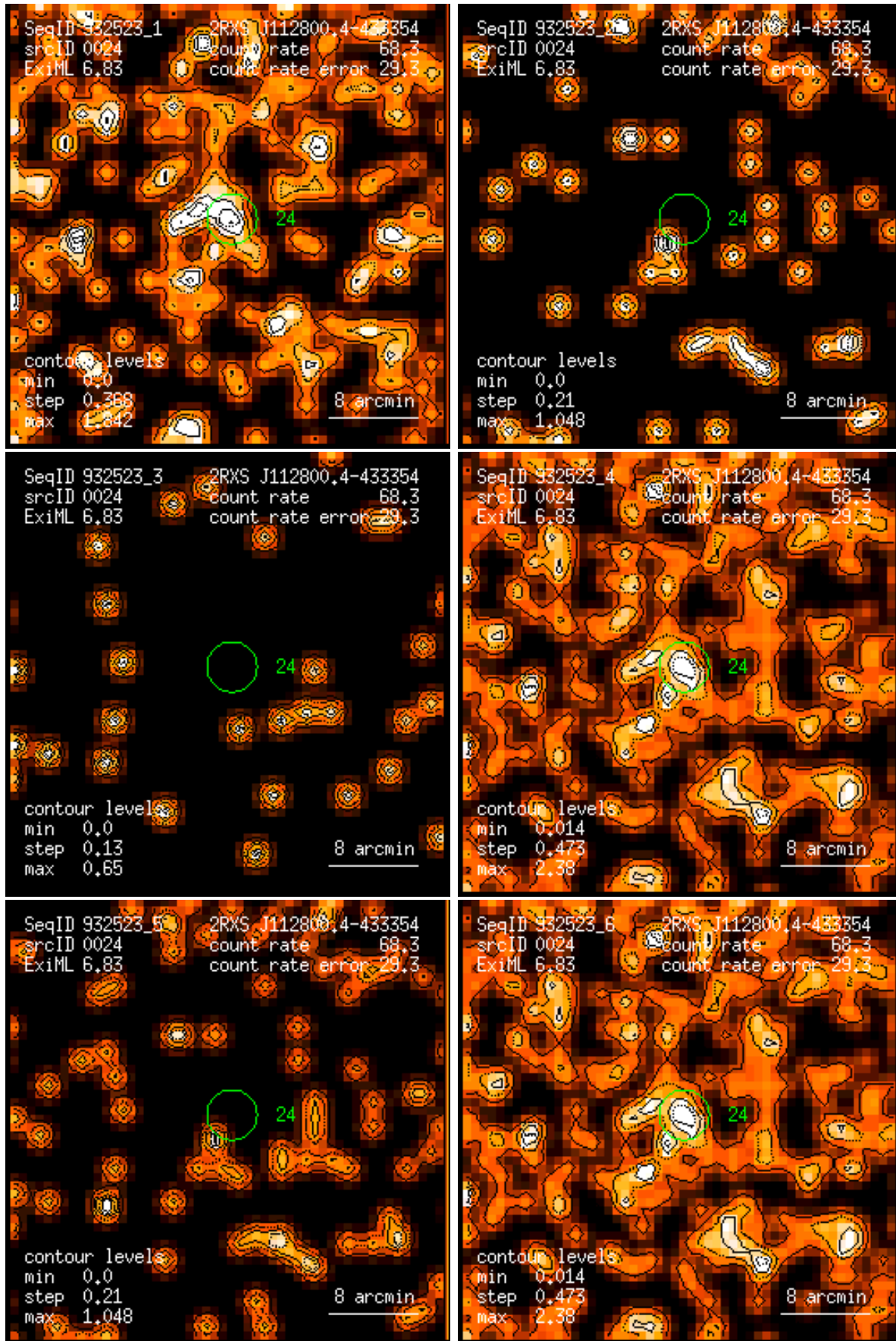
Figure 24: RASS 932523: detection 0024: band rate images, Gaussian filter: (1) PSPC channels 11 – 41, (2) 52 – 90, (3) 91 – 201, (4) 11 – 235, (5) 52 – 201, (6) 11 – 201. Broad band rates in counts/ks. Band rate contour levels in counts/ks/arcmin 2 .
