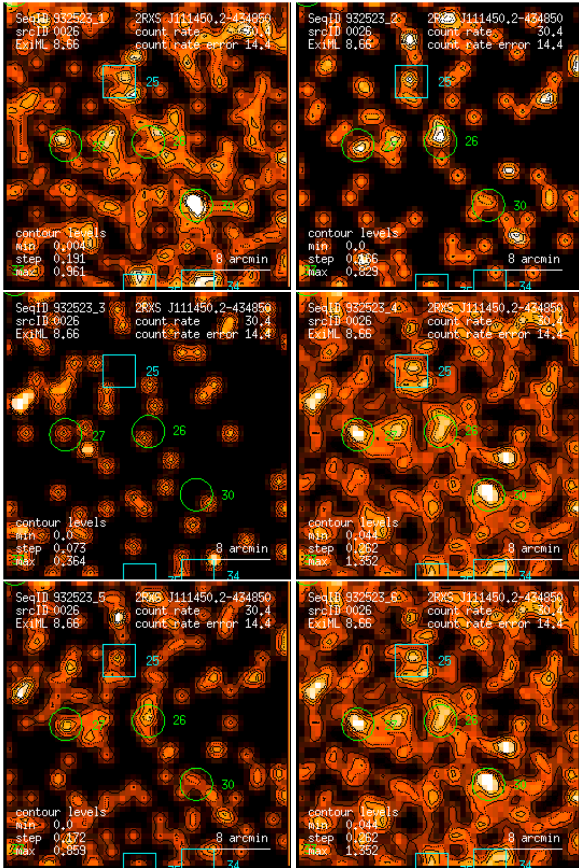
Figure 26: RASS 932523: detection 0026: band rate images, Gaussian filter: (1) PSPC channels 11 – 41, (2) 52 – 90, (3) 91 – 201, (4) 11 – 235, (5) 52 – 201, (6) 11 – 201. Broad band rates in counts/ks. Band rate contour levels in counts/ks/arcmin 2 .
