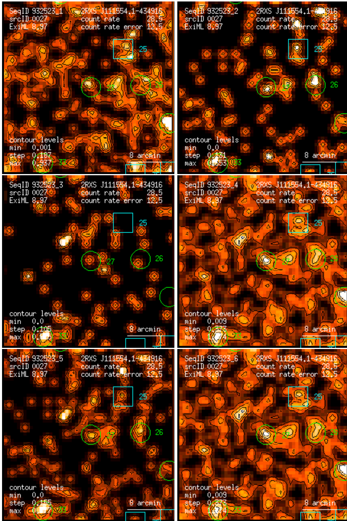
Figure 27: RASS 932523: detection 0027: band rate images, Gaussian filter: (1) PSPC channels 11 – 41, (2) 52 – 90, (3) 91 – 201, (4) 11 – 235, (5) 52 – 201, (6) 11 – 201. Broad band rates in counts/ks. Band rate contour levels in counts/ks/arcmin 2 .
