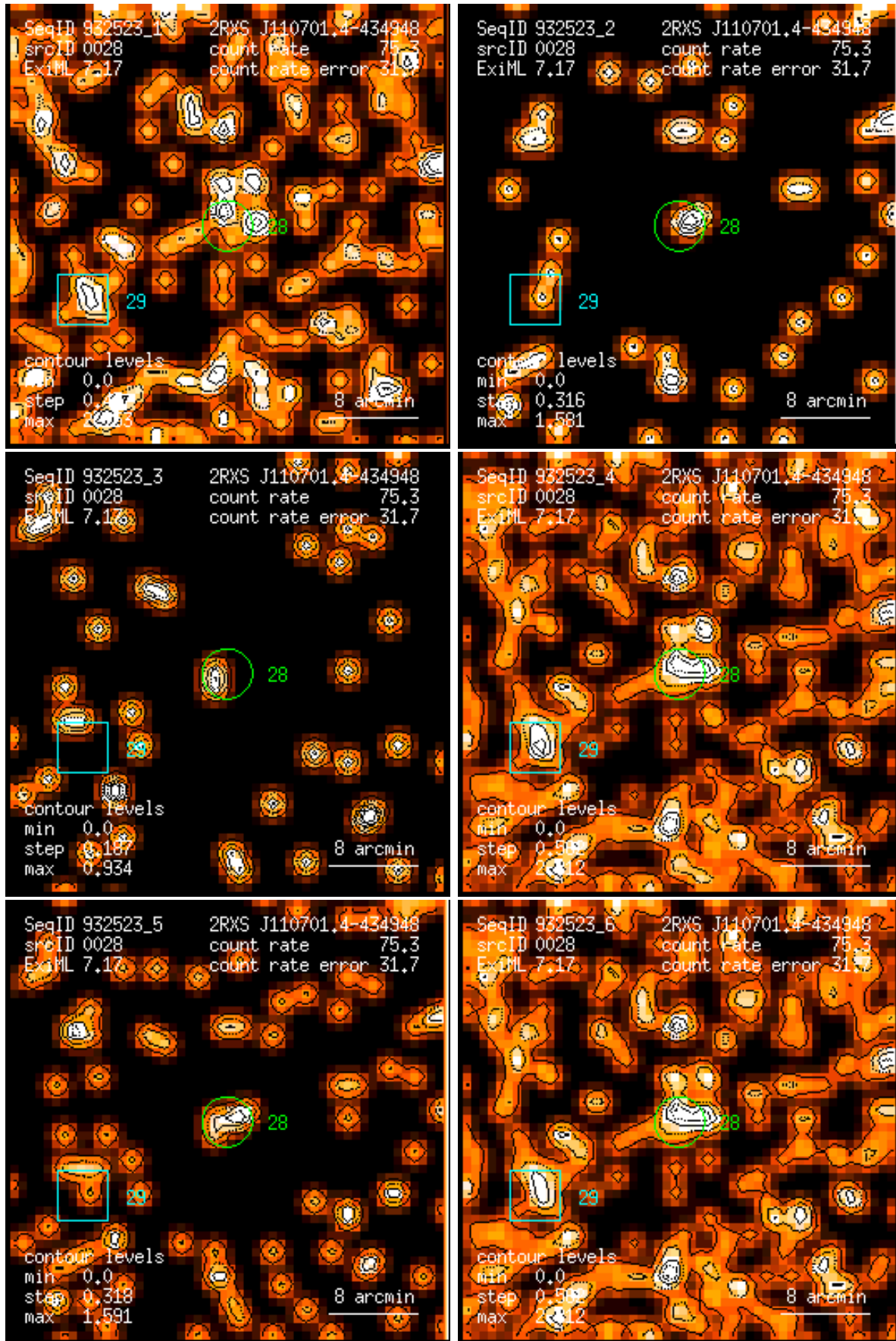
Figure 28: RASS 932523: detection 0028: band rate images, Gaussian filter: (1) PSPC channels 11 – 41, (2) 52 – 90, (3) 91 – 201, (4) 11 – 235, (5) 52 – 201, (6) 11 – 201. Broad band rates in counts/ks. Band rate contour levels in counts/ks/arcmin 2 .
