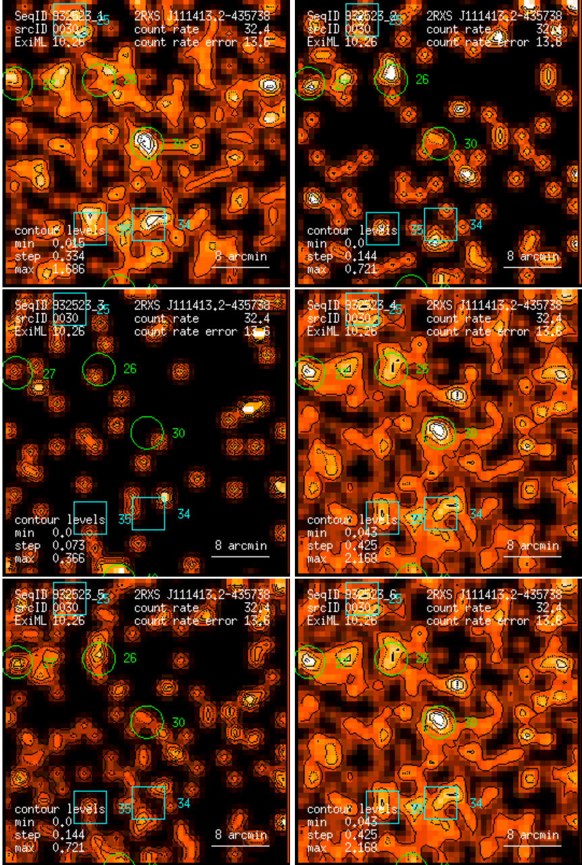
Figure 30: RASS 932523: detection 0030: band rate images, Gaussian filter: (1) PSPC channels 11 – 41, (2) 52 – 90, (3) 91 – 201, (4) 11 – 235, (5) 52 – 201, (6) 11 – 201. Broad band rates in counts/ks. Band rate contour levels in counts/ks/arcmin 2 .
