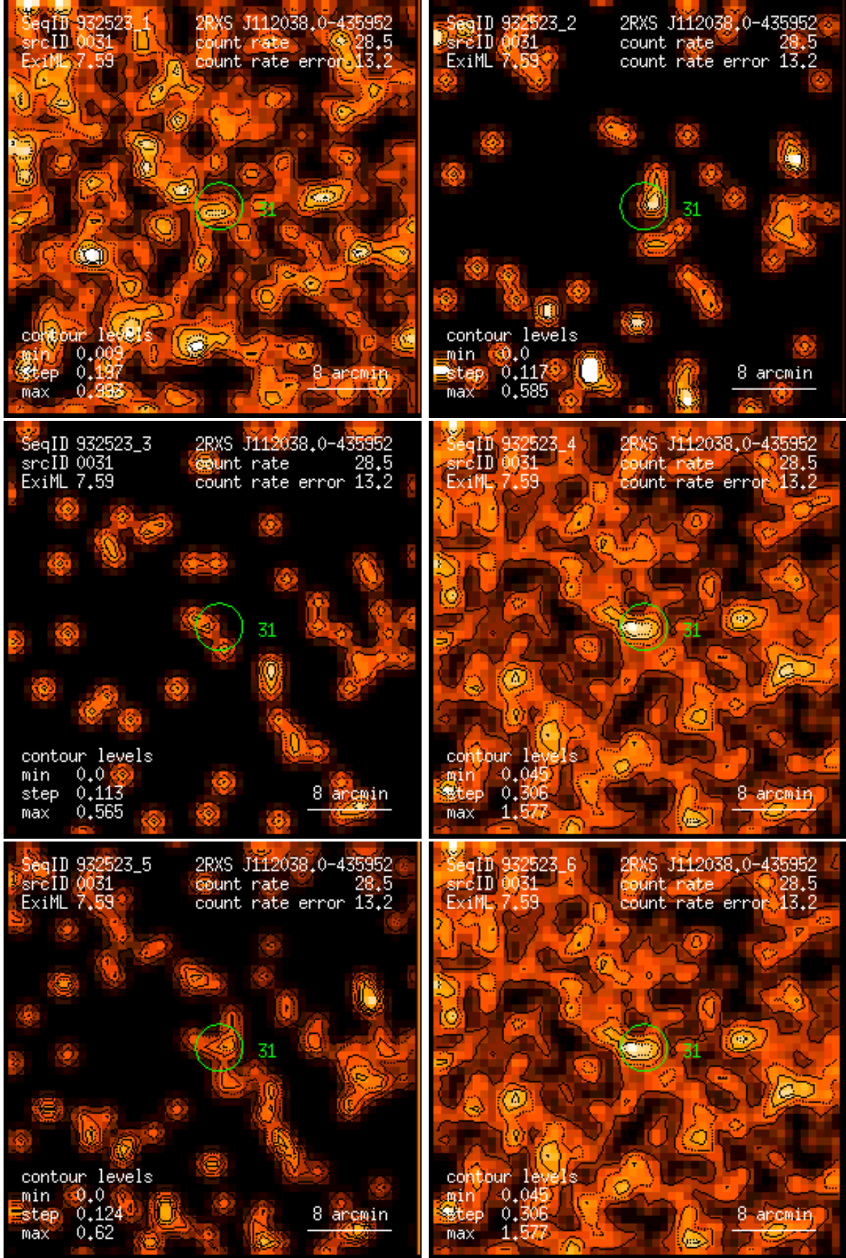
Figure 31: RASS 932523: detection 0031: band rate images, Gaussian filter: (1) PSPC channels 11 – 41, (2) 52 – 90, (3) 91 – 201, (4) 11 – 235, (5) 52 – 201, (6) 11 – 201. Broad band rates in counts/ks. Band rate contour levels in counts/ks/arcmin 2 .
