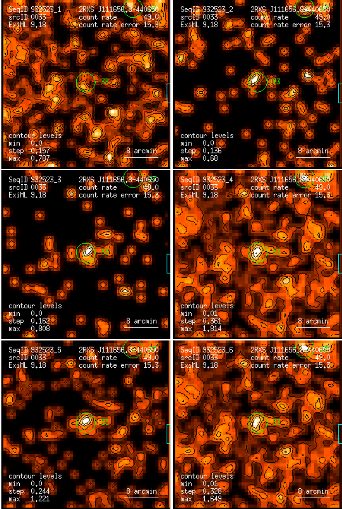
Figure 33: RASS 932523: detection 0033: band rate images, Gaussian filter: (1) PSPC channels 11 – 41, (2) 52 – 90, (3) 91 – 201, (4) 11 – 235, (5) 52 – 201, (6) 11 – 201. Broad band rates in counts/ks. Band rate contour levels in counts/ks/arcmin 2 .
