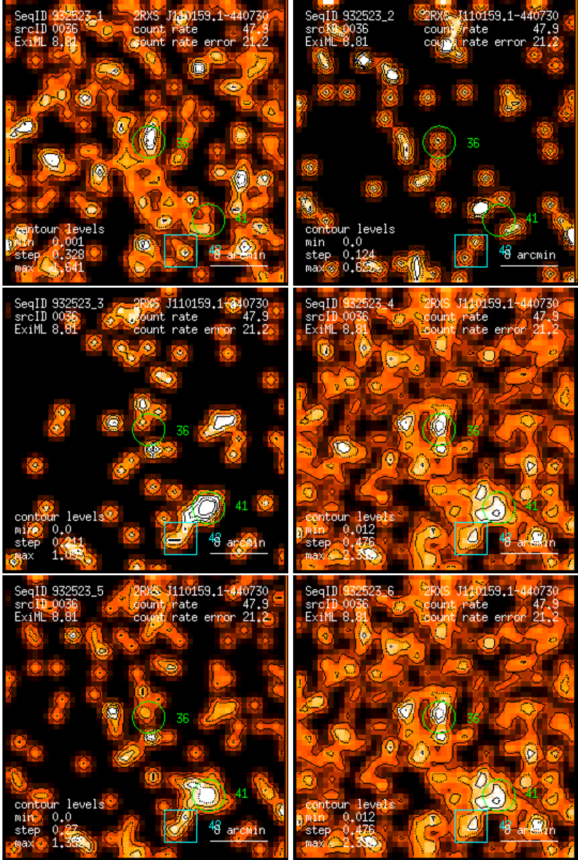
Figure 36: RASS 932523: detection 0036: band rate images, Gaussian filter: (1) PSPC channels 11 – 41, (2) 52 – 90, (3) 91 – 201, (4) 11 – 235, (5) 52 – 201, (6) 11 – 201. Broad band rates in counts/ks. Band rate contour levels in counts/ks/arcmin 2 .
