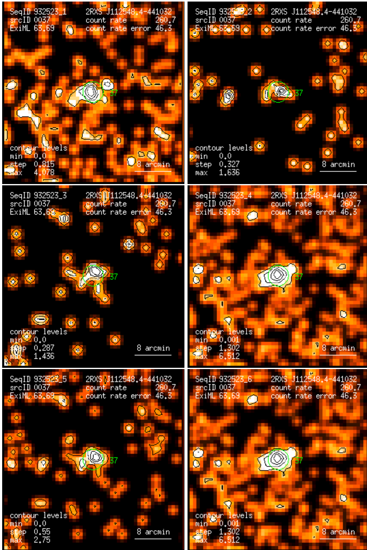
Figure 37: RASS 932523: detection 0037: band rate images, Gaussian filter: (1) PSPC channels 11 – 41, (2) 52 – 90, (3) 91 – 201, (4) 11 – 235, (5) 52 – 201, (6) 11 – 201. Broad band rates in counts/ks. Band rate contour levels in counts/ks/arcmin 2 .
