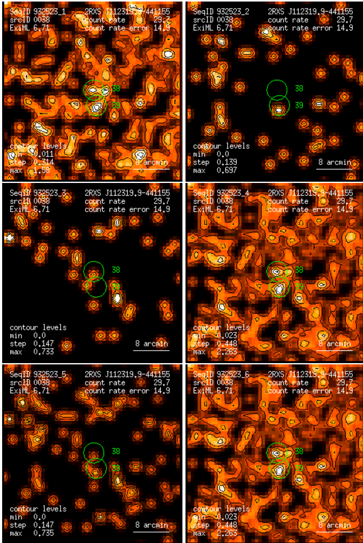
Figure 38: RASS 932523: detection 0038: band rate images, Gaussian filter: (1) PSPC channels 11 – 41, (2) 52 – 90, (3) 91 – 201, (4) 11 – 235, (5) 52 – 201, (6) 11 – 201. Broad band rates in counts/ks. Band rate contour levels in counts/ks/arcmin 2 .
