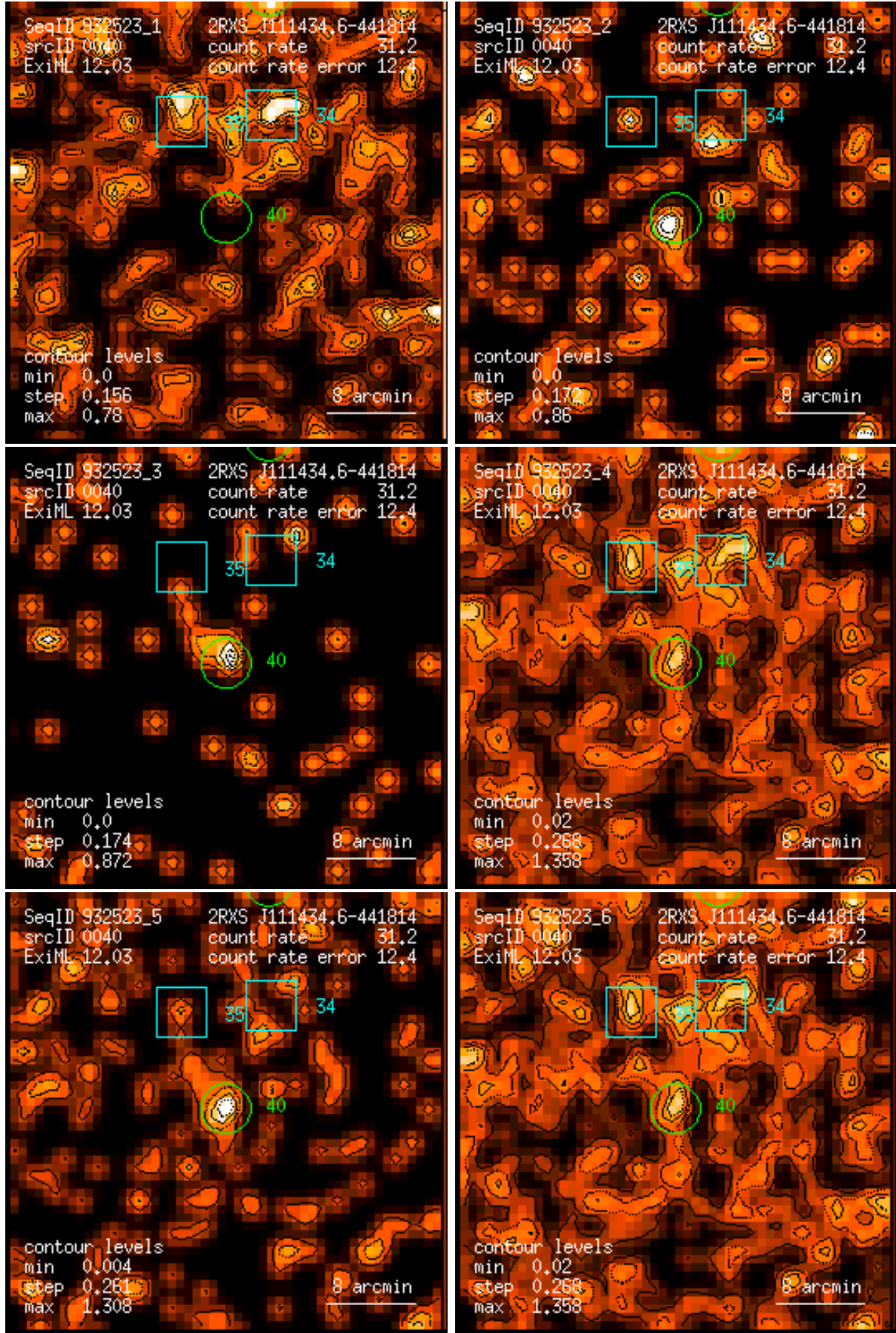
Figure 40: RASS 932523: detection 0040: band rate images, Gaussian filter: (1) PSPC channels 11 – 41, (2) 52 – 90, (3) 91 – 201, (4) 11 – 235, (5) 52 – 201, (6) 11 – 201. Broad band rates in counts/ks. Band rate contour levels in counts/ks/arcmin 2 .
