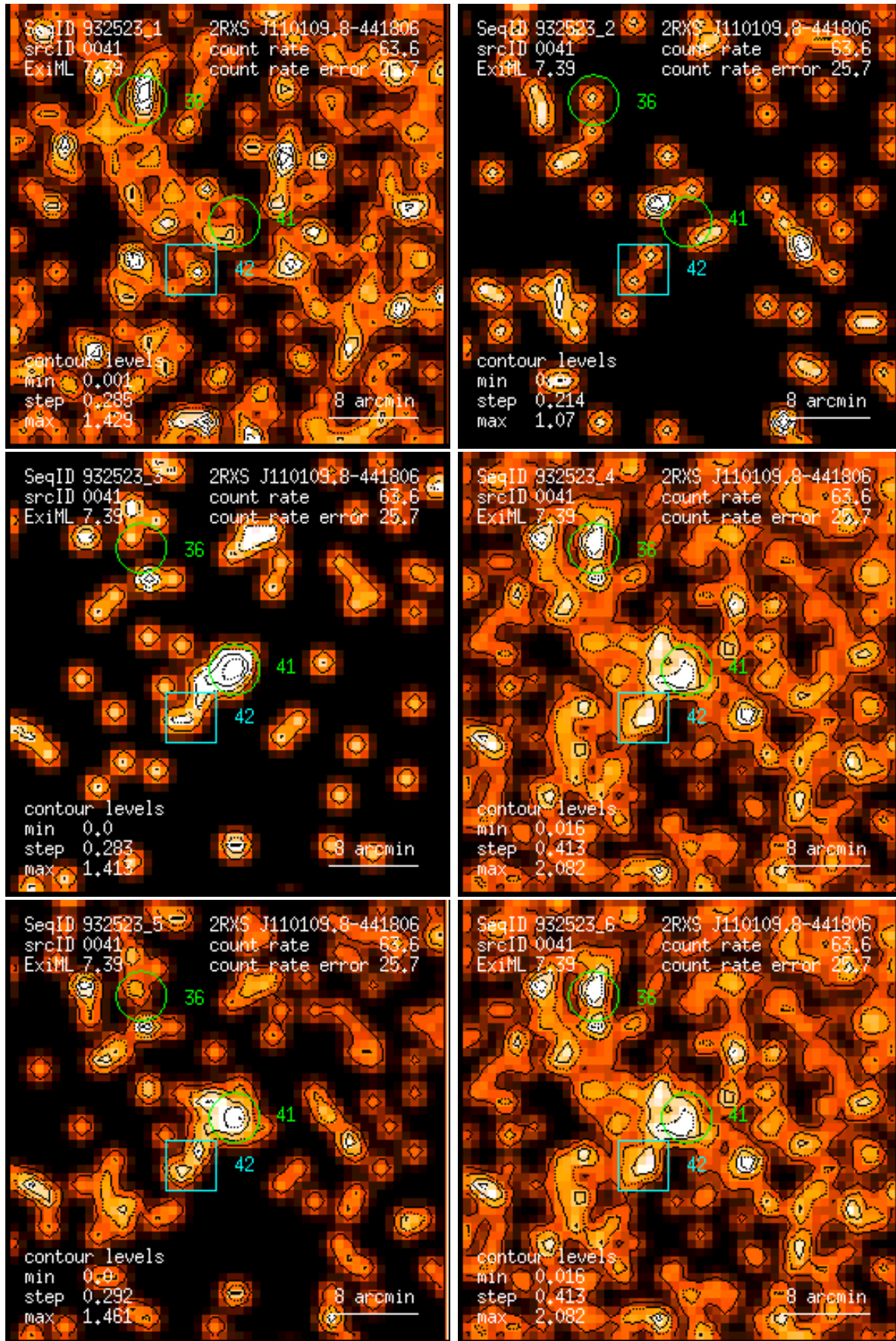
Figure 41: RASS 932523: detection 0041: band rate images, Gaussian filter: (1) PSPC channels 11 – 41, (2) 52 – 90, (3) 91 – 201, (4) 11 – 235, (5) 52 – 201, (6) 11 – 201. Broad band rates in counts/ks. Band rate contour levels in counts/ks/arcmin 2 .
