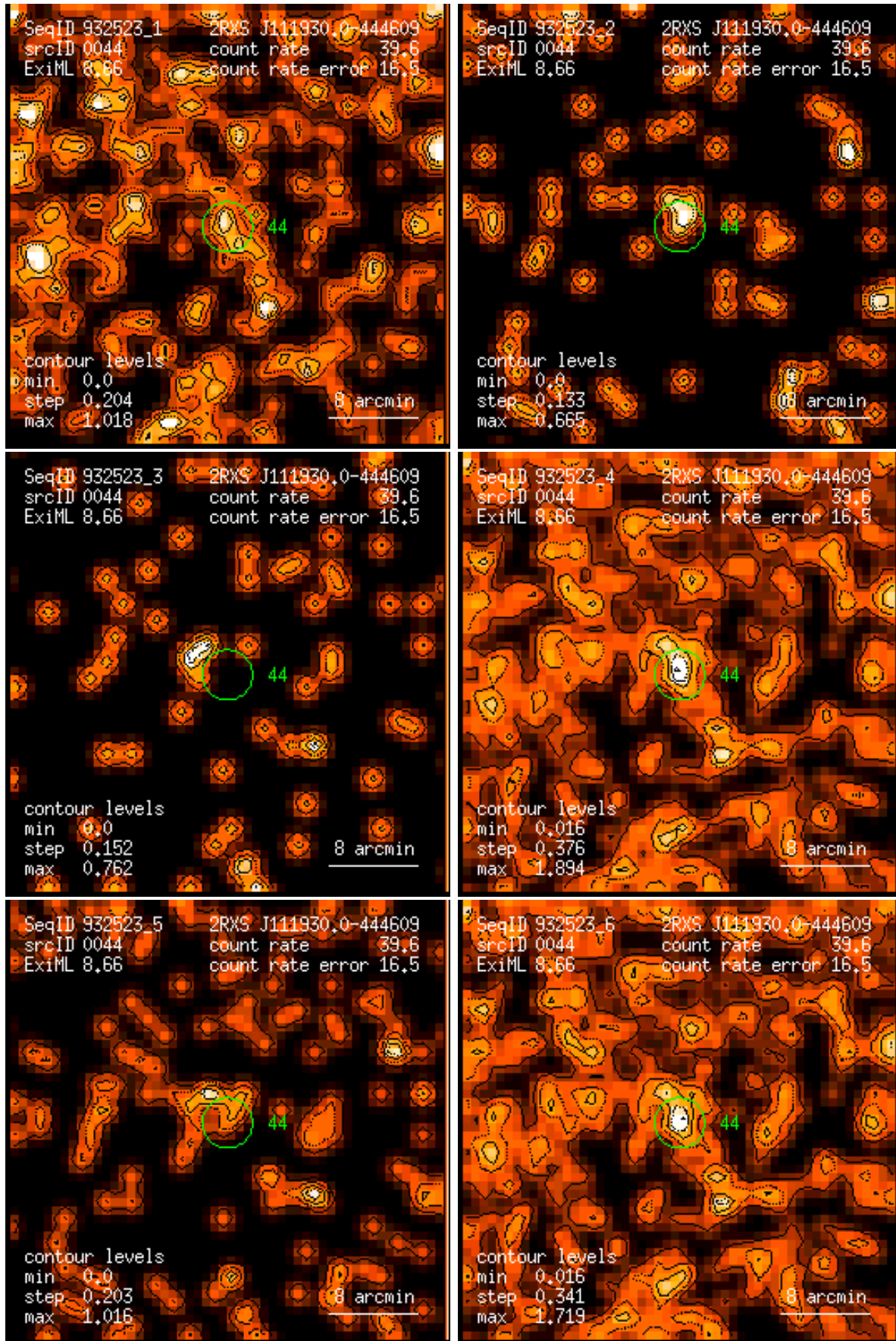
Figure 44: RASS 932523: detection 0044: band rate images, Gaussian filter: (1) PSPC channels 11 – 41, (2) 52 – 90, (3) 91 – 201, (4) 11 – 235, (5) 52 – 201, (6) 11 – 201. Broad band rates in counts/ks. Band rate contour levels in counts/ks/arcmin 2 .
