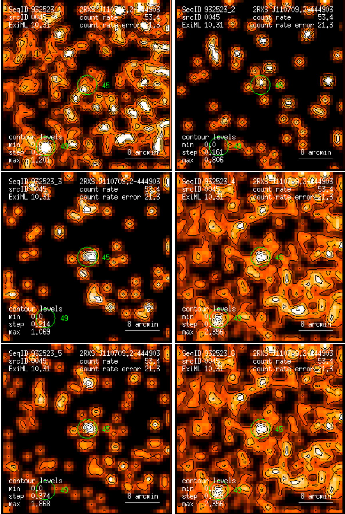
Figure 45: RASS 932523: detection 0045: band rate images, Gaussian filter: (1) PSPC channels 11 – 41, (2) 52 – 90, (3) 91 – 201, (4) 11 – 235, (5) 52 – 201, (6) 11 – 201. Broad band rates in counts/ks. Band rate contour levels in counts/ks/arcmin 2 .
