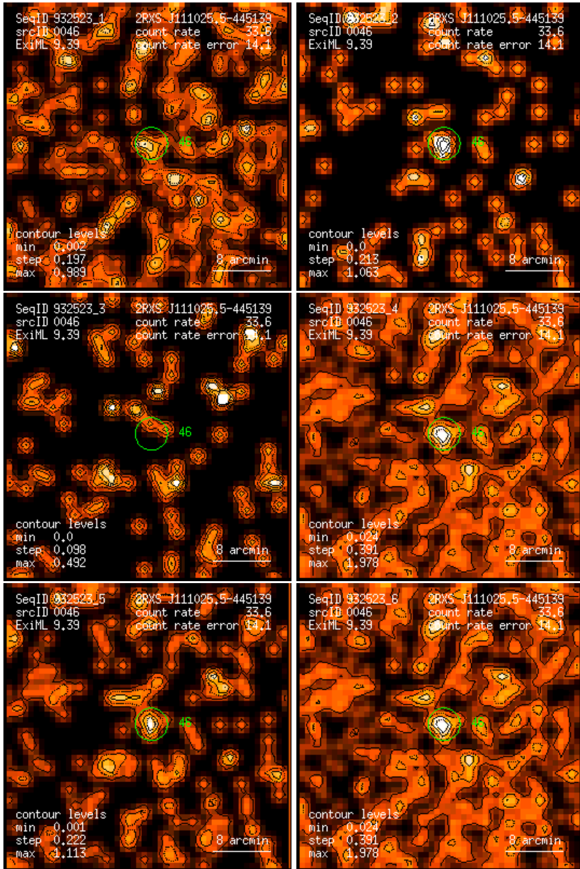
Figure 46: RASS 932523: detection 0046: band rate images, Gaussian filter: (1) PSPC channels 11 – 41, (2) 52 – 90, (3) 91 – 201, (4) 11 – 235, (5) 52 – 201, (6) 11 – 201. Broad band rates in counts/ks. Band rate contour levels in counts/ks/arcmin 2 .
