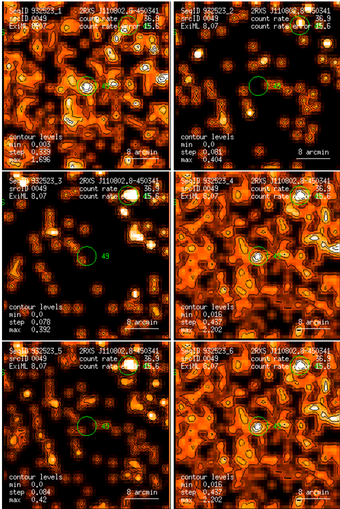
Figure 49: RASS 932523: detection 0049: band rate images, Gaussian filter: (1) PSPC channels 11 – 41, (2) 52 – 90, (3) 91 – 201, (4) 11 – 235, (5) 52 – 201, (6) 11 – 201. Broad band rates in counts/ks. Band rate contour levels in counts/ks/arcmin 2 .
