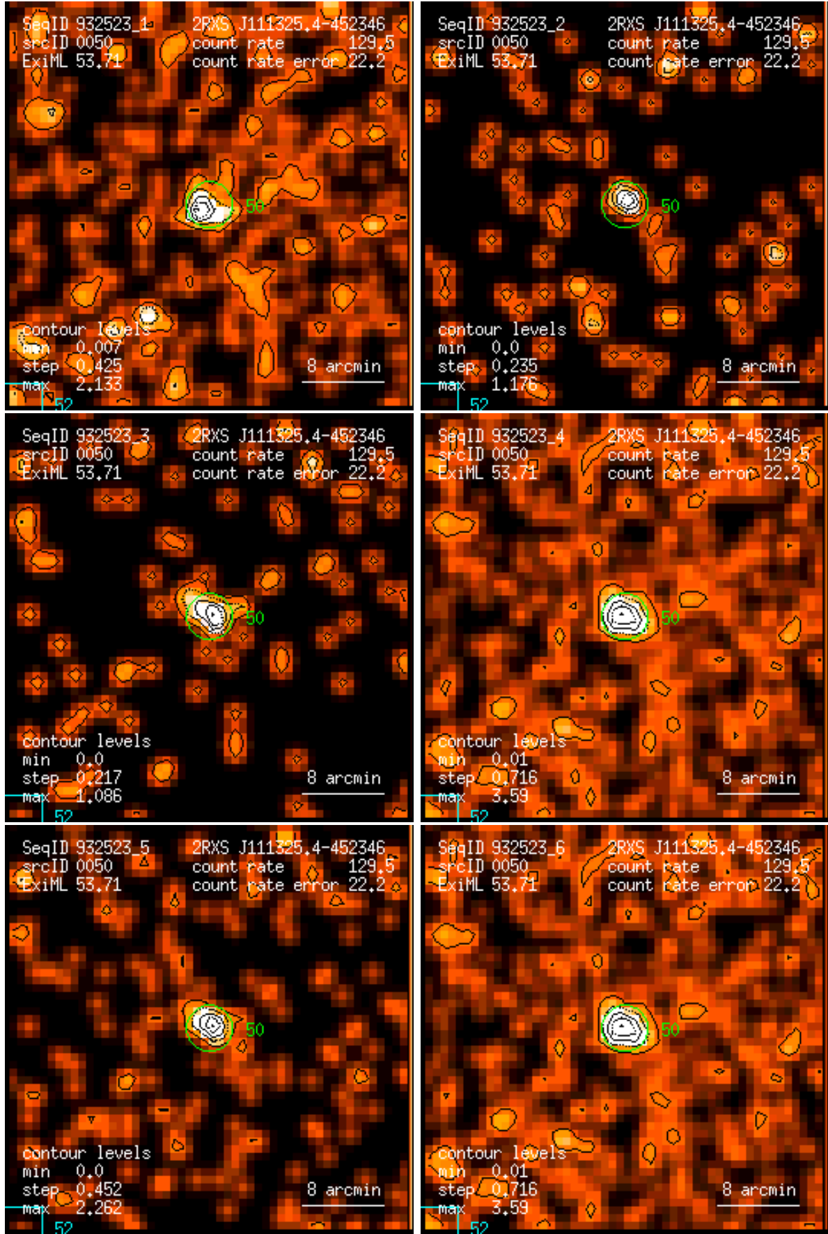
Figure 50: RASS 932523: detection 0050: band rate images, Gaussian filter: (1) PSPC channels 11 – 41, (2) 52 – 90, (3) 91 – 201, (4) 11 – 235, (5) 52 – 201, (6) 11 – 201. Broad band rates in counts/ks. Band rate contour levels in counts/ks/arcmin 2 .
