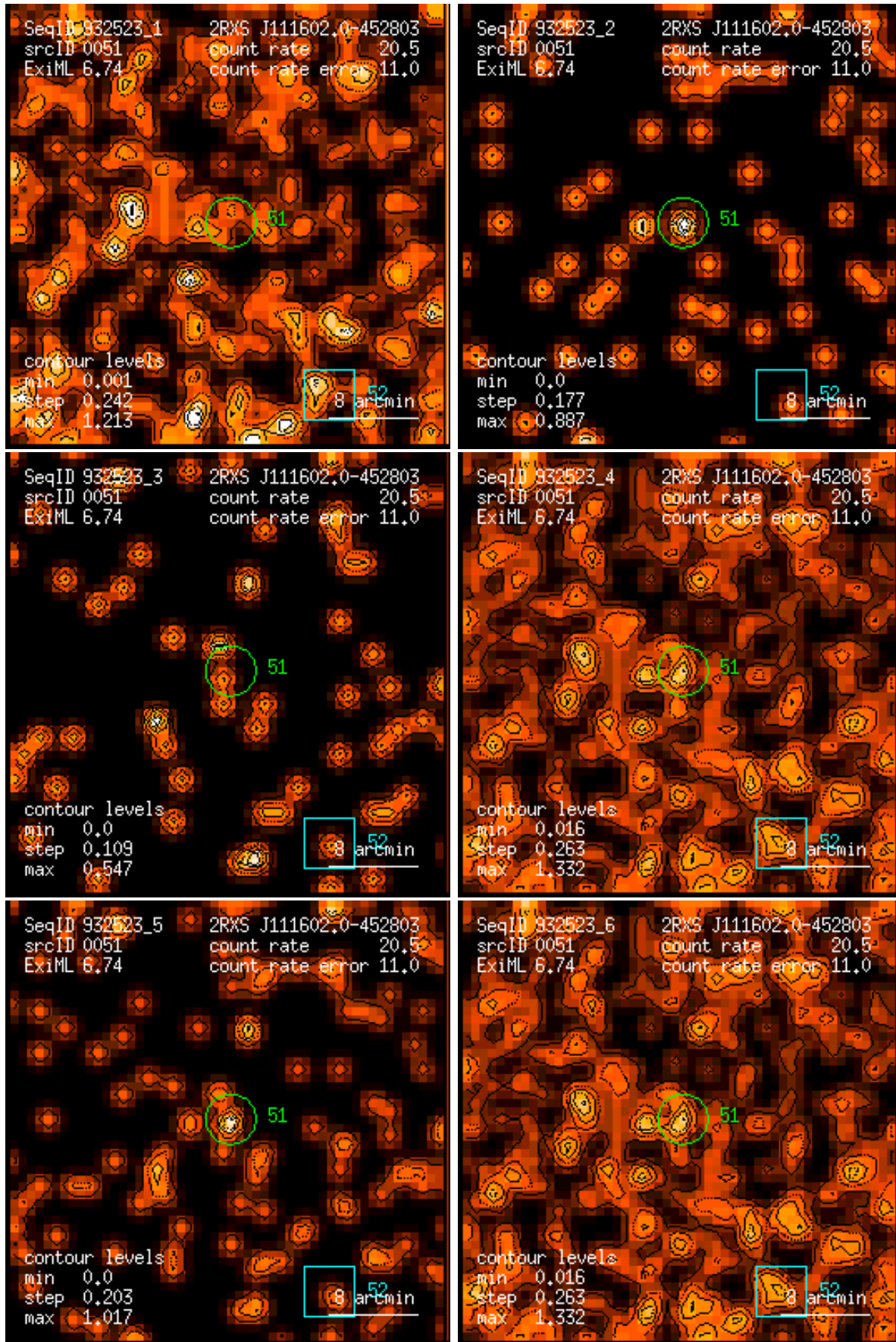
Figure 51: RASS 932523: detection 0051: band rate images, Gaussian filter: (1) PSPC channels 11 – 41, (2) 52 – 90, (3) 91 – 201, (4) 11 – 235, (5) 52 – 201, (6) 11 – 201. Broad band rates in counts/ks. Band rate contour levels in counts/ks/arcmin 2 .
