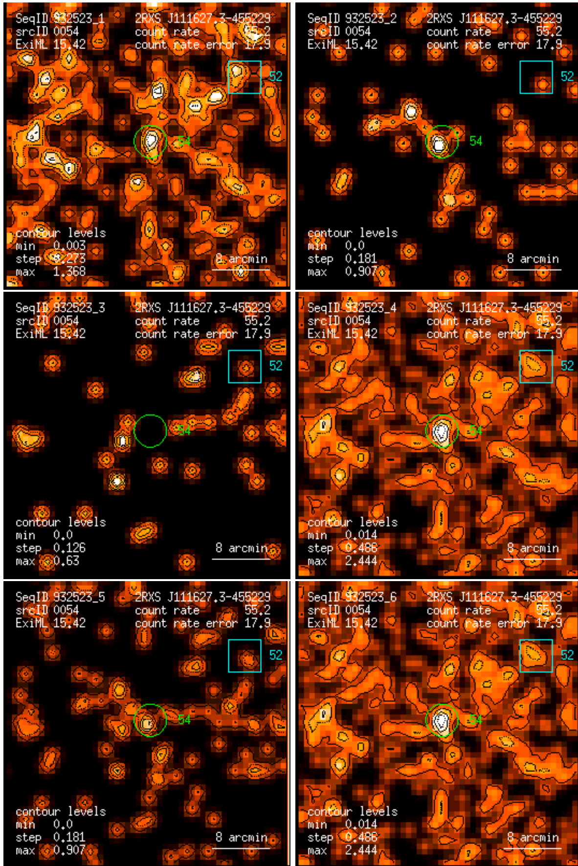
Figure 54: RASS 932523: detection 0054: band rate images, Gaussian filter: (1) PSPC channels 11 – 41, (2) 52 – 90, (3) 91 – 201, (4) 11 – 235, (5) 52 – 201, (6) 11 – 201. Broad band rates in counts/ks. Band rate contour levels in counts/ks/arcmin 2 .
