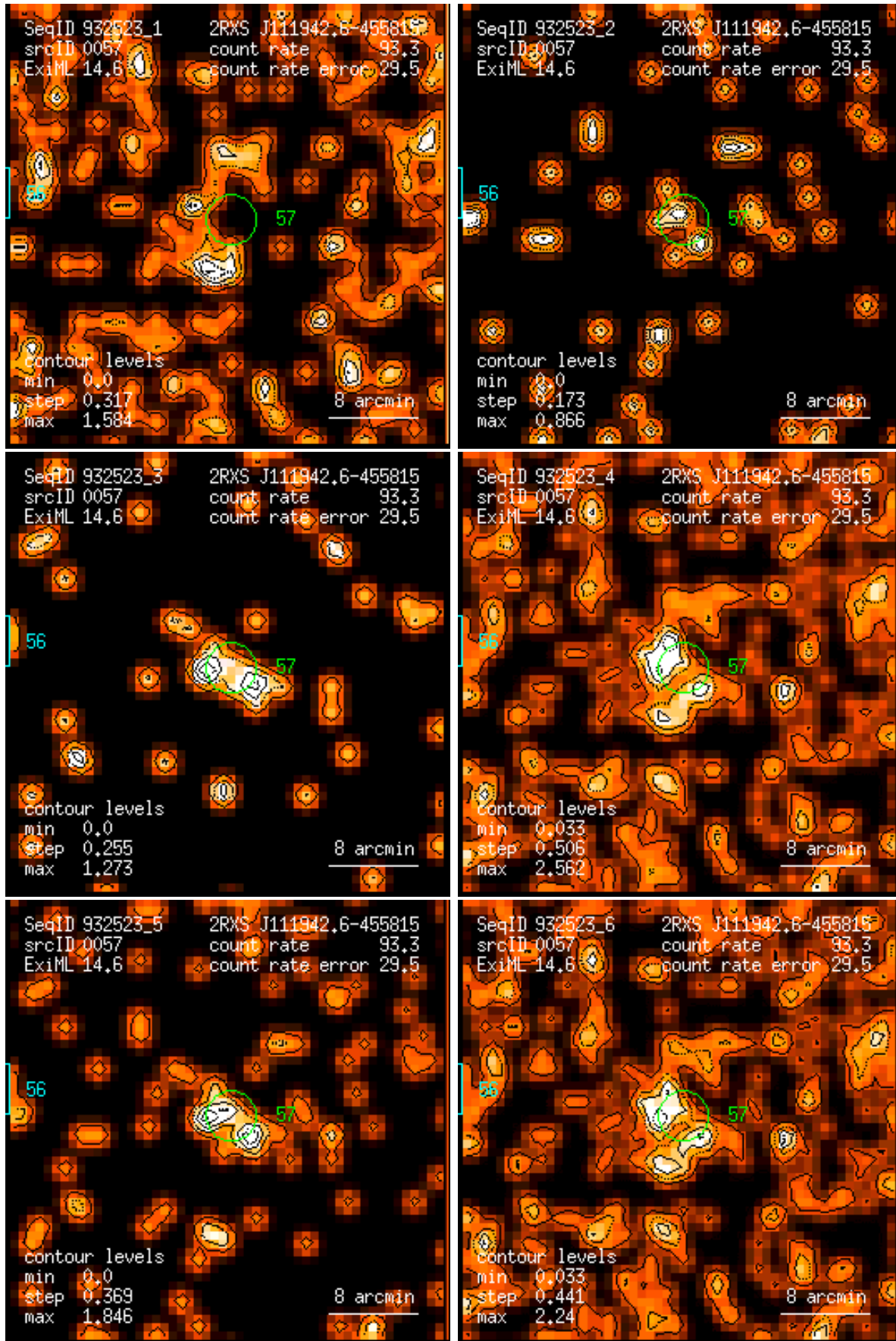
Figure 57: RASS 932523: detection 0057: band rate images, Gaussian filter: (1) PSPC channels 11 – 41, (2) 52 – 90, (3) 91 – 201, (4) 11 – 235, (5) 52 – 201, (6) 11 – 201. Broad band rates in counts/ks. Band rate contour levels in counts/ks/arcmin 2 .
