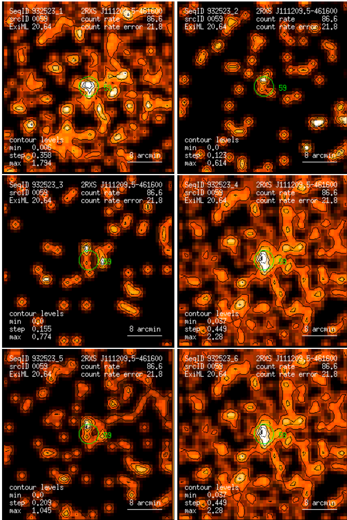
Figure 59: RASS 932523: detection 0059: band rate images, Gaussian filter: (1) PSPC channels 11 – 41, (2) 52 – 90, (3) 91 – 201, (4) 11 – 235, (5) 52 – 201, (6) 11 – 201. Broad band rates in counts/ks. Band rate contour levels in counts/ks/arcmin 2 .
