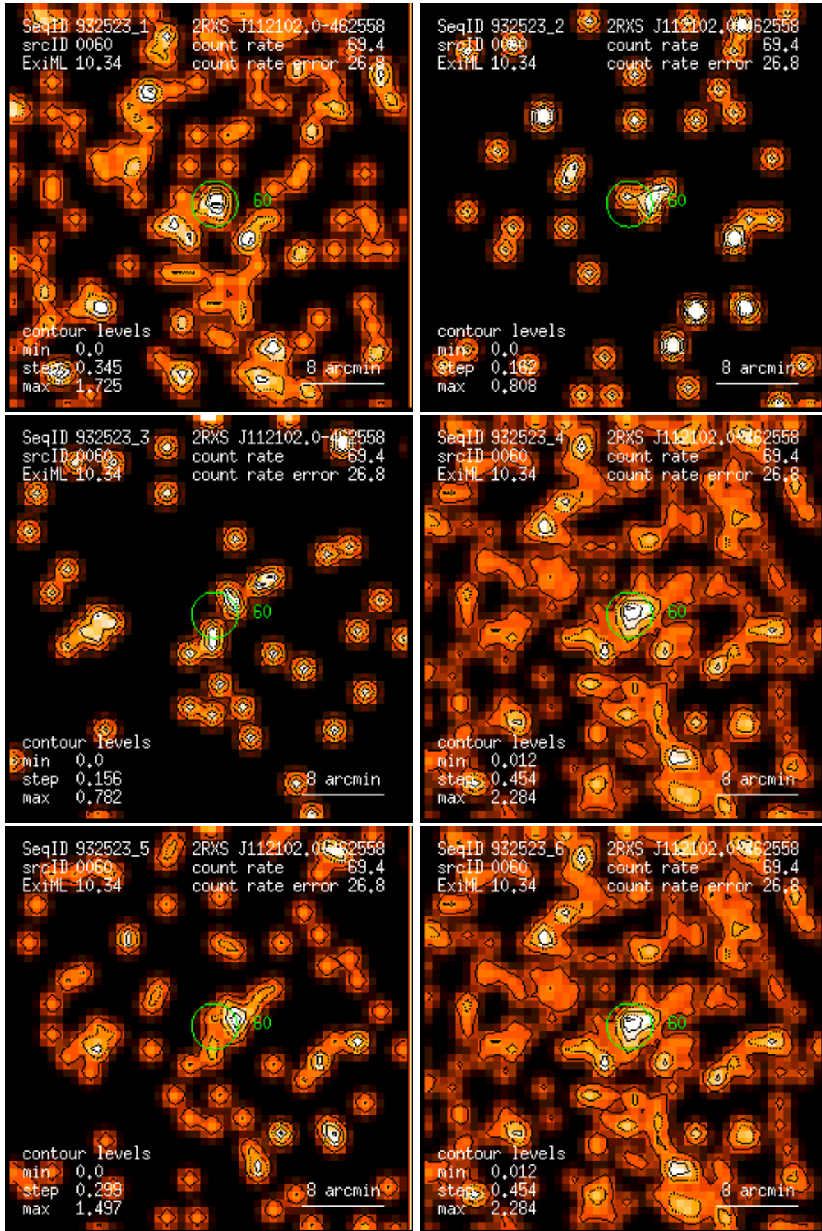
Figure 60: RASS 932523: detection 0060: band rate images, Gaussian filter: (1) PSPC channels 11 – 41, (2) 52 – 90, (3) 91 – 201, (4) 11 – 235, (5) 52 – 201, (6) 11 – 201. Broad band rates in counts/ks. Band rate contour levels in counts/ks/arcmin 2 .
