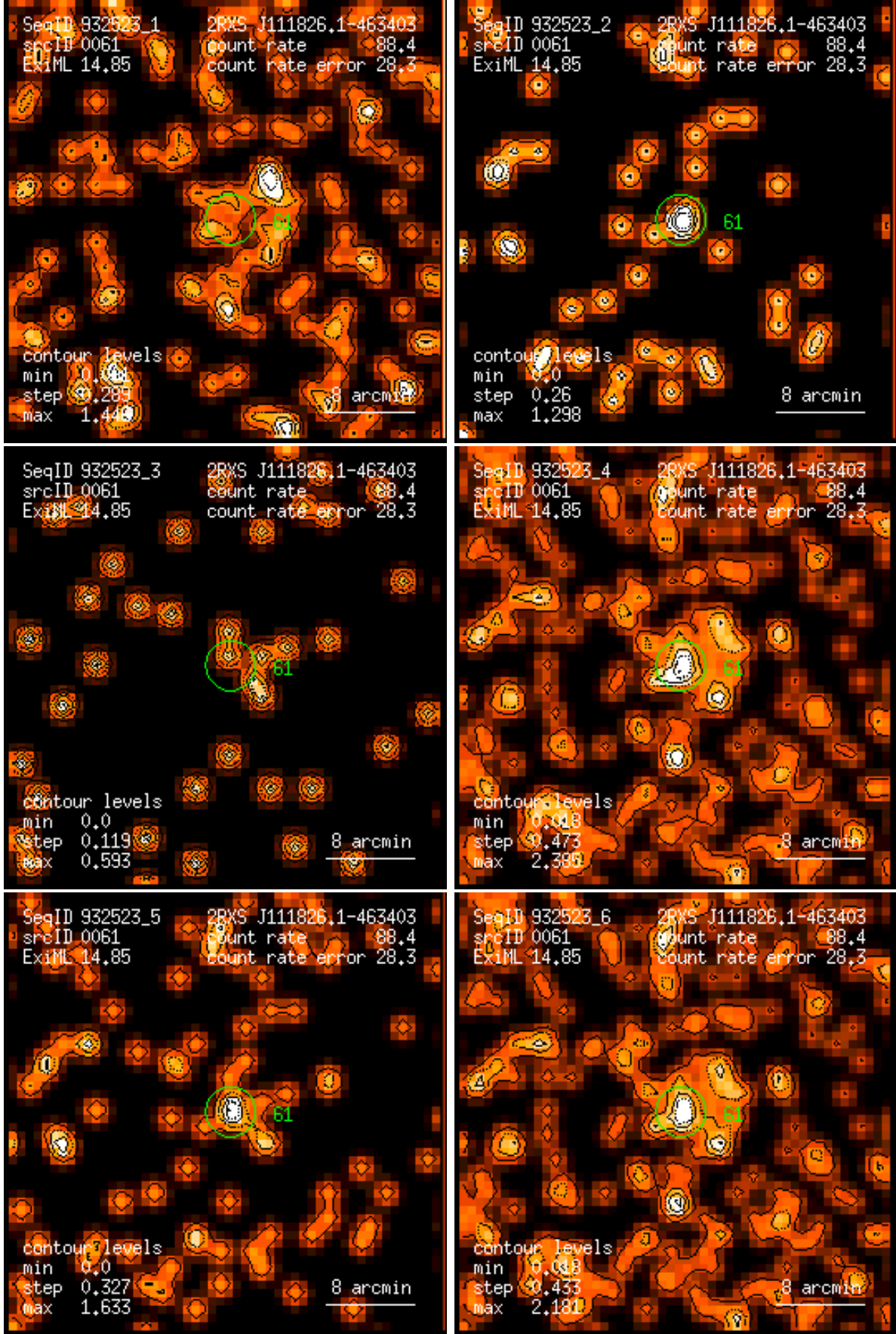
Figure 61: RASS 932523: detection 0061: band rate images, Gaussian filter: (1) PSPC channels 11 – 41, (2) 52 – 90, (3) 91 – 201, (4) 11 – 235, (5) 52 – 201, (6) 11 – 201. Broad band rates in counts/ks. Band rate contour levels in counts/ks/arcmin 2 .
