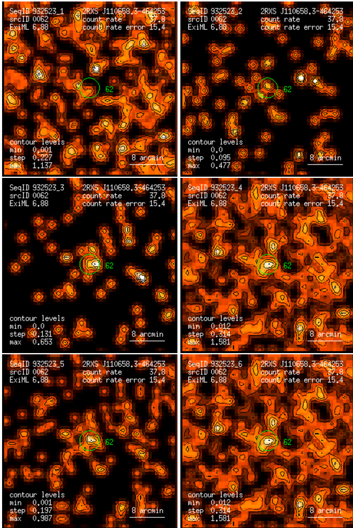
Figure 62: RASS 932523: detection 0062: band rate images, Gaussian filter: (1) PSPC channels 11 – 41, (2) 52 – 90, (3) 91 – 201, (4) 11 – 235, (5) 52 – 201, (6) 11 – 201. Broad band rates in counts/ks. Band rate contour levels in counts/ks/arcmin 2 .
