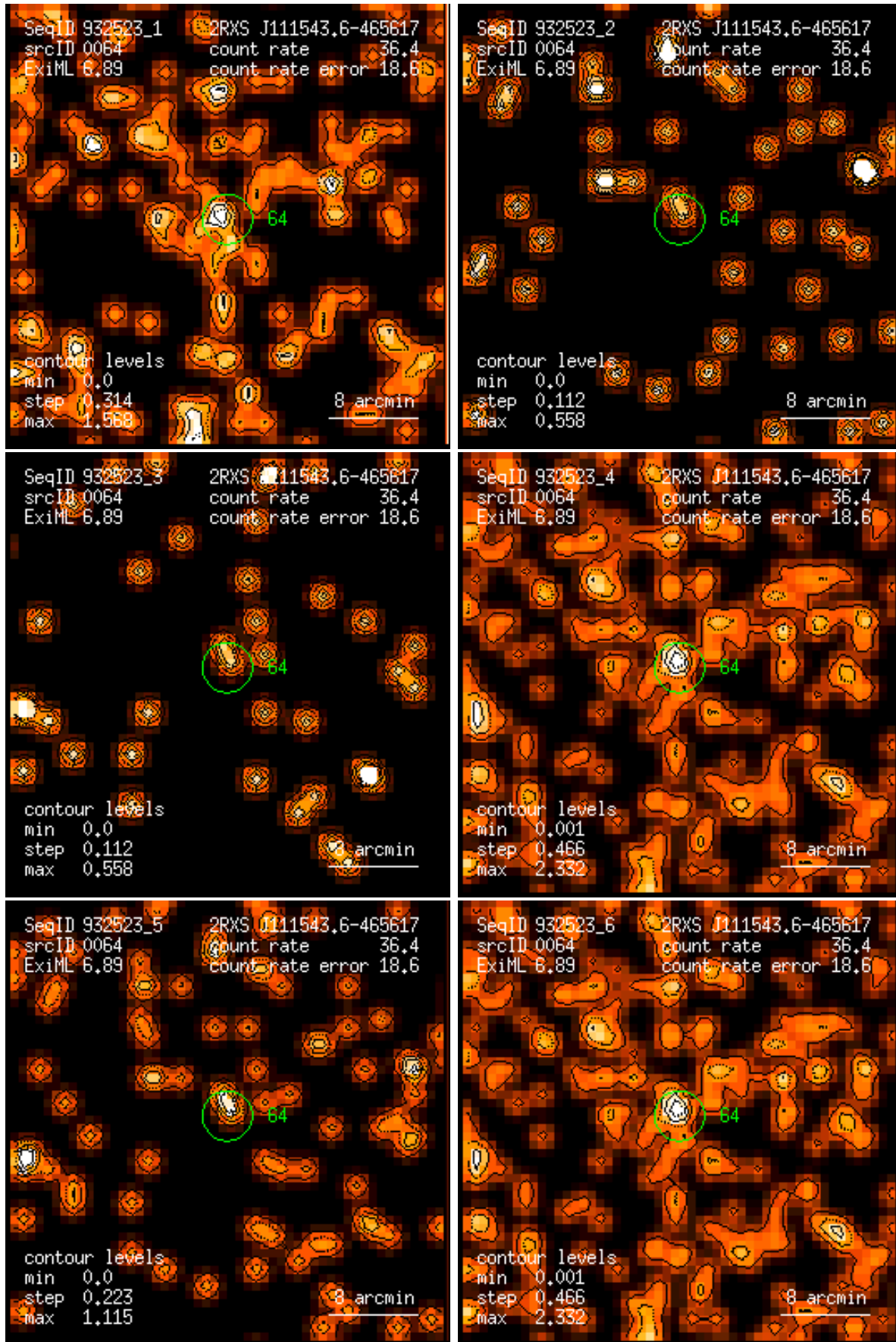
Figure 64: RASS 932523: detection 0064: band rate images, Gaussian filter: (1) PSPC channels 11 – 41, (2) 52 – 90, (3) 91 – 201, (4) 11 – 235, (5) 52 – 201, (6) 11 – 201. Broad band rates in counts/ks. Band rate contour levels in counts/ks/arcmin 2 .
