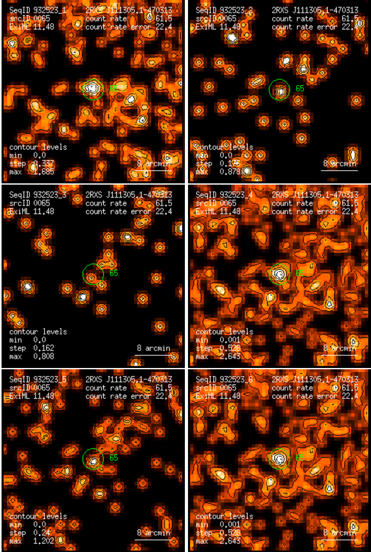
Figure 65: RASS 932523: detection 0065: band rate images, Gaussian filter: (1) PSPC channels 11 – 41, (2) 52 – 90, (3) 91 – 201, (4) 11 – 235, (5) 52 – 201, (6) 11 – 201. Broad band rates in counts/ks. Band rate contour levels in counts/ks/arcmin 2 .
