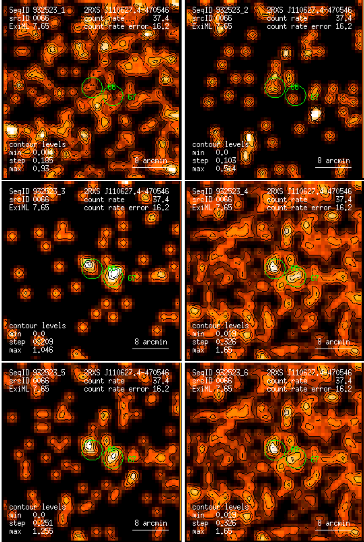
Figure 66: RASS 932523: detection 0066: band rate images, Gaussian filter: (1) PSPC channels 11 – 41, (2) 52 – 90, (3) 91 – 201, (4) 11 – 235, (5) 52 – 201, (6) 11 – 201. Broad band rates in counts/ks. Band rate contour levels in counts/ks/arcmin 2 .
