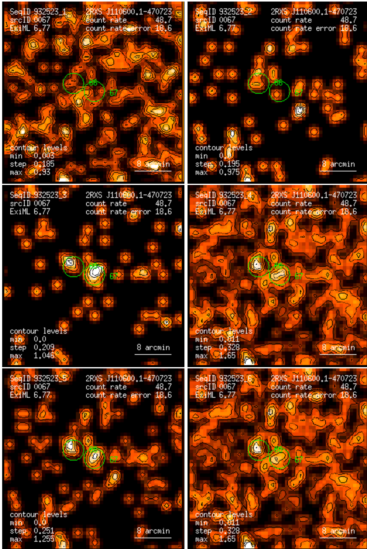
Figure 67: RASS 932523: detection 0067: band rate images, Gaussian filter: (1) PSPC channels 11 – 41, (2) 52 – 90, (3) 91 – 201, (4) 11 – 235, (5) 52 – 201, (6) 11 – 201. Broad band rates in counts/ks. Band rate contour levels in counts/ks/arcmin 2 .
