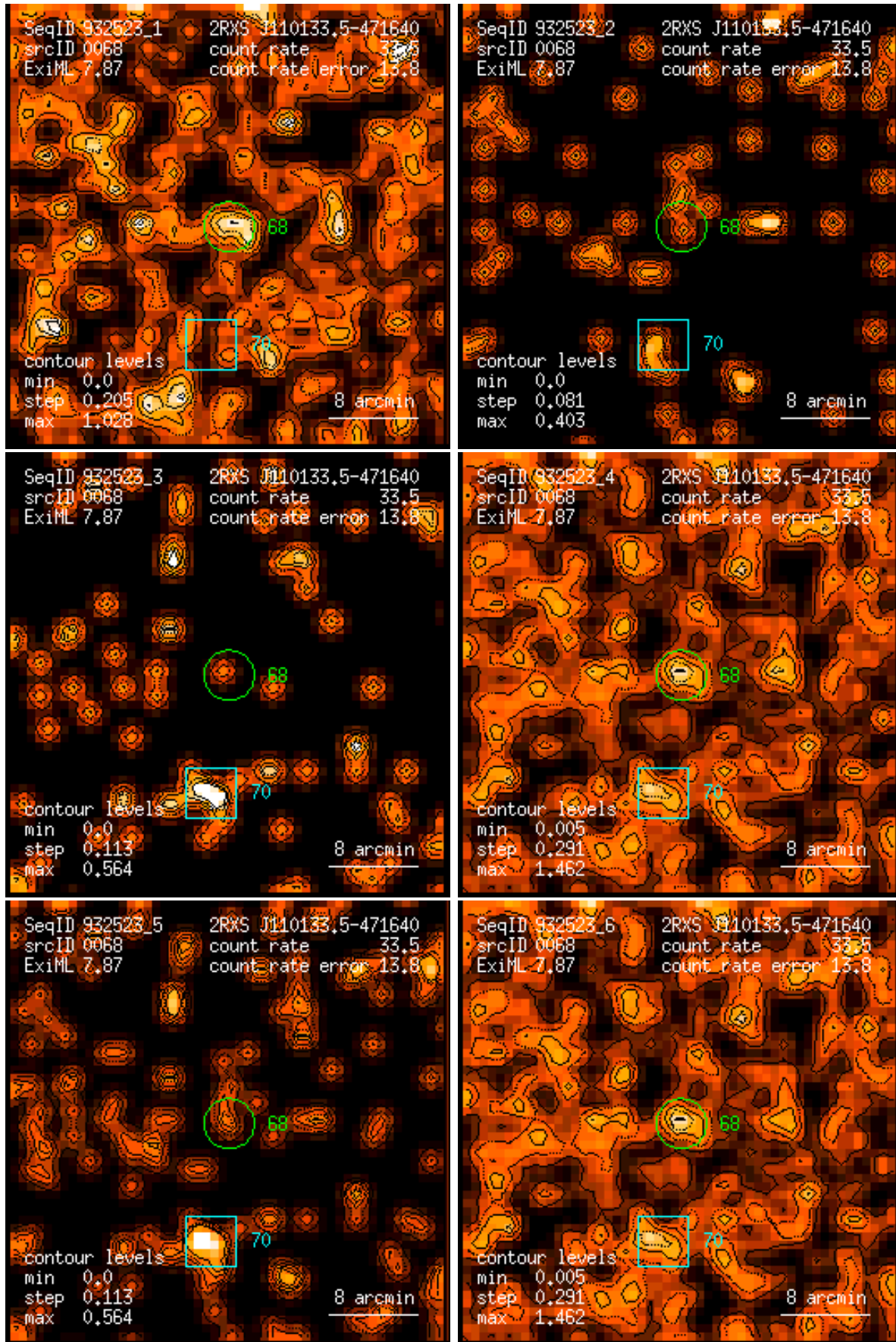
Figure 68: RASS 932523: detection 0068: band rate images, Gaussian filter: (1) PSPC channels 11 – 41, (2) 52 – 90, (3) 91 – 201, (4) 11 – 235, (5) 52 – 201, (6) 11 – 201. Broad band rates in counts/ks. Band rate contour levels in counts/ks/arcmin 2 .
