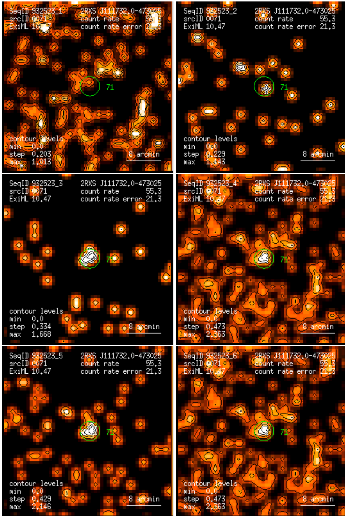
Figure 71: RASS 932523: detection 0071: band rate images, Gaussian filter: (1) PSPC channels 11 – 41, (2) 52 – 90, (3) 91 – 201, (4) 11 – 235, (5) 52 – 201, (6) 11 – 201. Broad band rates in counts/ks. Band rate contour levels in counts/ks/arcmin 2 .
