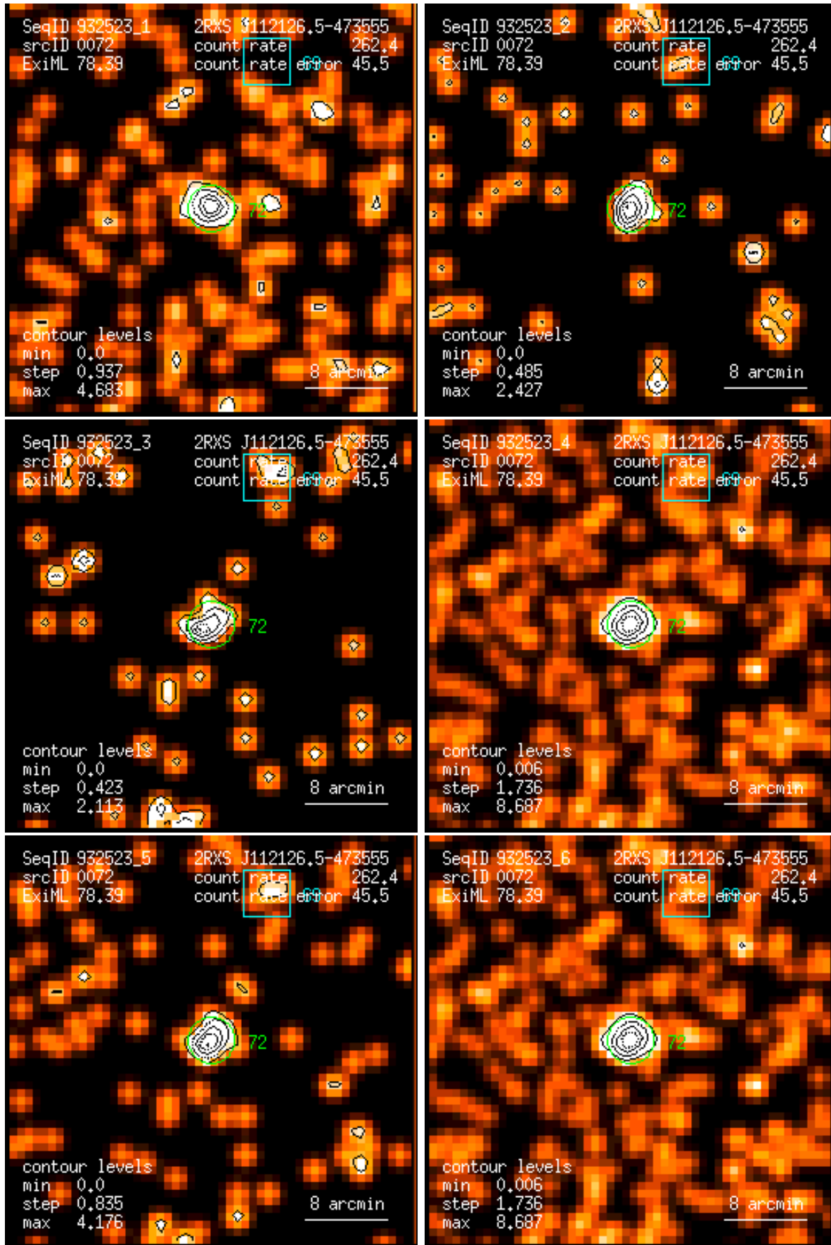
Figure 72: RASS 932523: detection 0072: band rate images, Gaussian filter: (1) PSPC channels 11 – 41, (2) 52 – 90, (3) 91 – 201, (4) 11 – 235, (5) 52 – 201, (6) 11 – 201. Broad band rates in counts/ks. Band rate contour levels in counts/ks/arcmin 2 .
