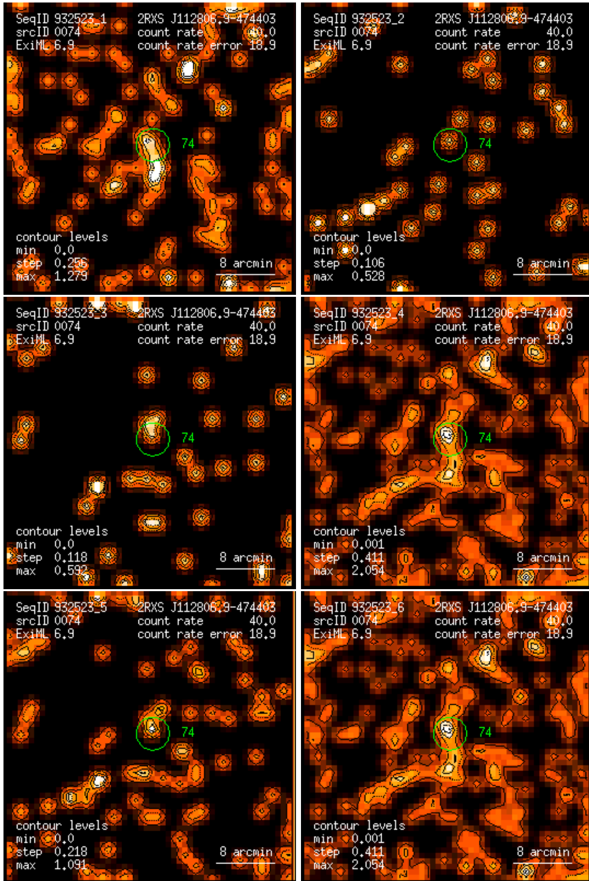
Figure 74: RASS 932523: detection 0074: band rate images, Gaussian filter: (1) PSPC channels 11 – 41, (2) 52 – 90, (3) 91 – 201, (4) 11 – 235, (5) 52 – 201, (6) 11 – 201. Broad band rates in counts/ks. Band rate contour levels in counts/ks/arcmin 2 .
