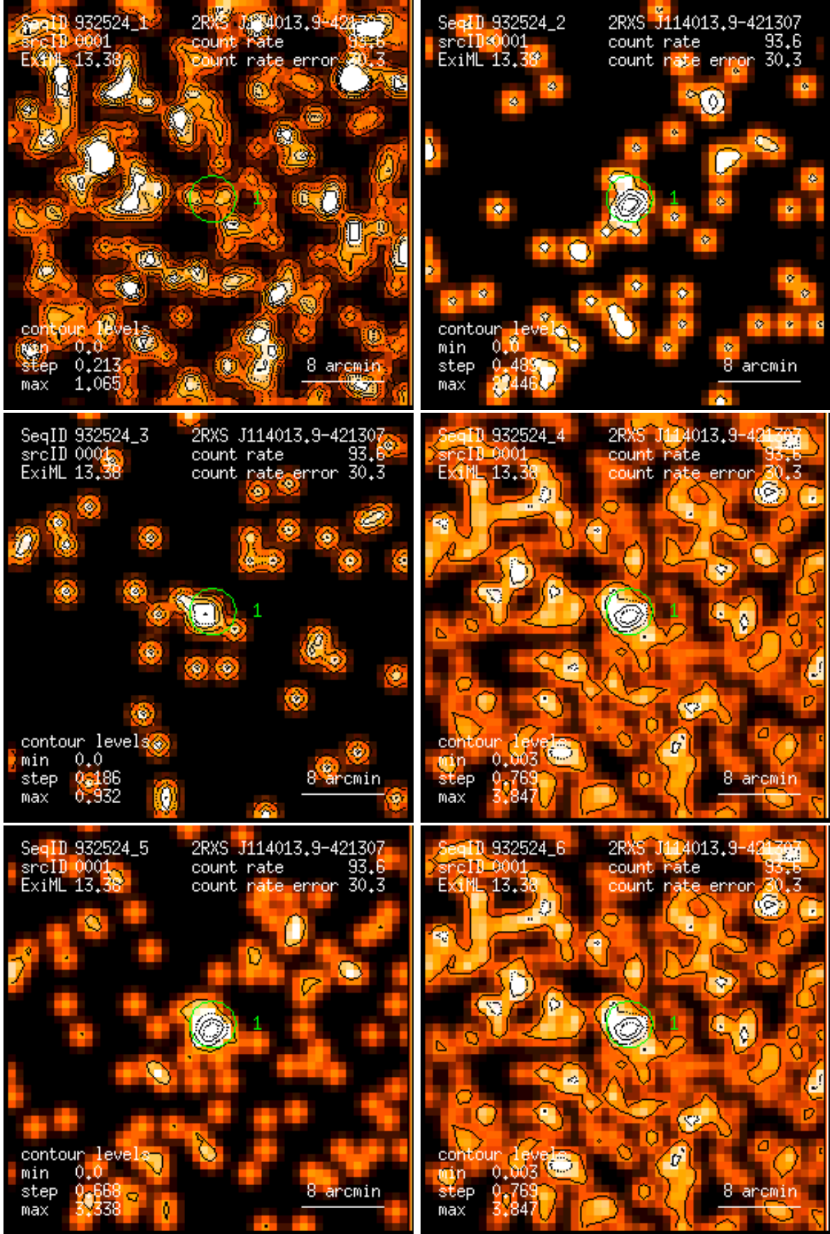
Figure 1: RASS 932524: detection 0001: band rate images, Gaussian filter: (1) PSPC channels 11 – 41, (2) 52 – 90, (3) 91 – 201, (4) 11 – 235, (5) 52 – 201, (6) 11 – 201. Broad band rates in counts/ks. Band rate contour levels in counts/ks/arcmin 2 .
