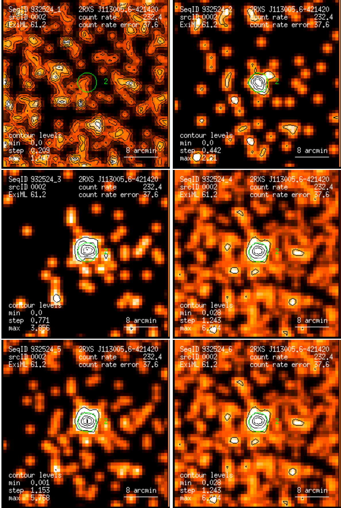
Figure 2: RASS 932524: detection 0002: band rate images, Gaussian filter: (1) PSPC channels 11 – 41, (2) 52 – 90, (3) 91 – 201, (4) 11 – 235, (5) 52 – 201, (6) 11 – 201. Broad band rates in counts/ks. Band rate contour levels in counts/ks/arcmin 2 .
