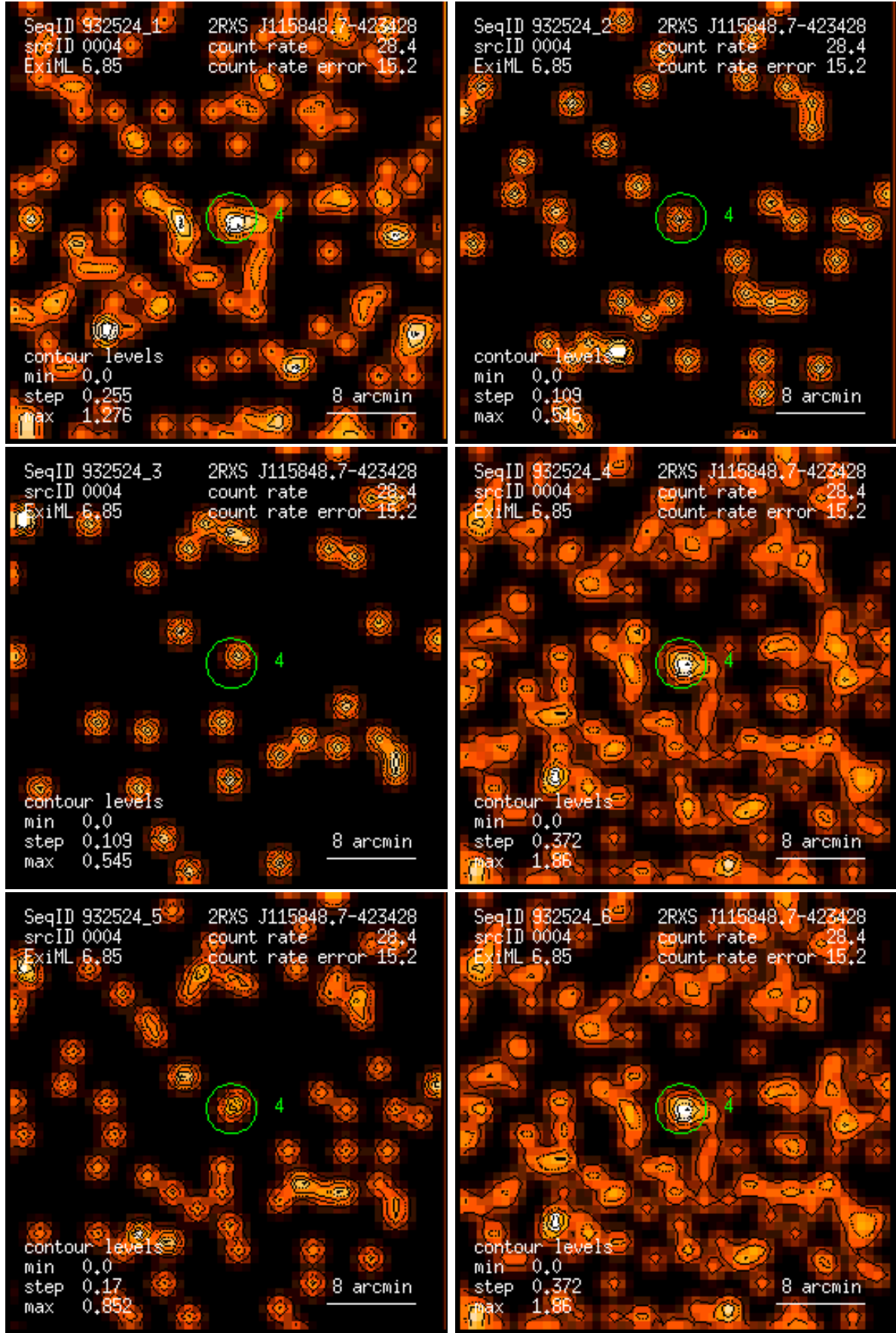
Figure 4: RASS 932524: detection 0004: band rate images, Gaussian filter: (1) PSPC channels 11 – 41, (2) 52 – 90, (3) 91 – 201, (4) 11 – 235, (5) 52 – 201, (6) 11 – 201. Broad band rates in counts/ks. Band rate contour levels in counts/ks/arcmin 2 .
