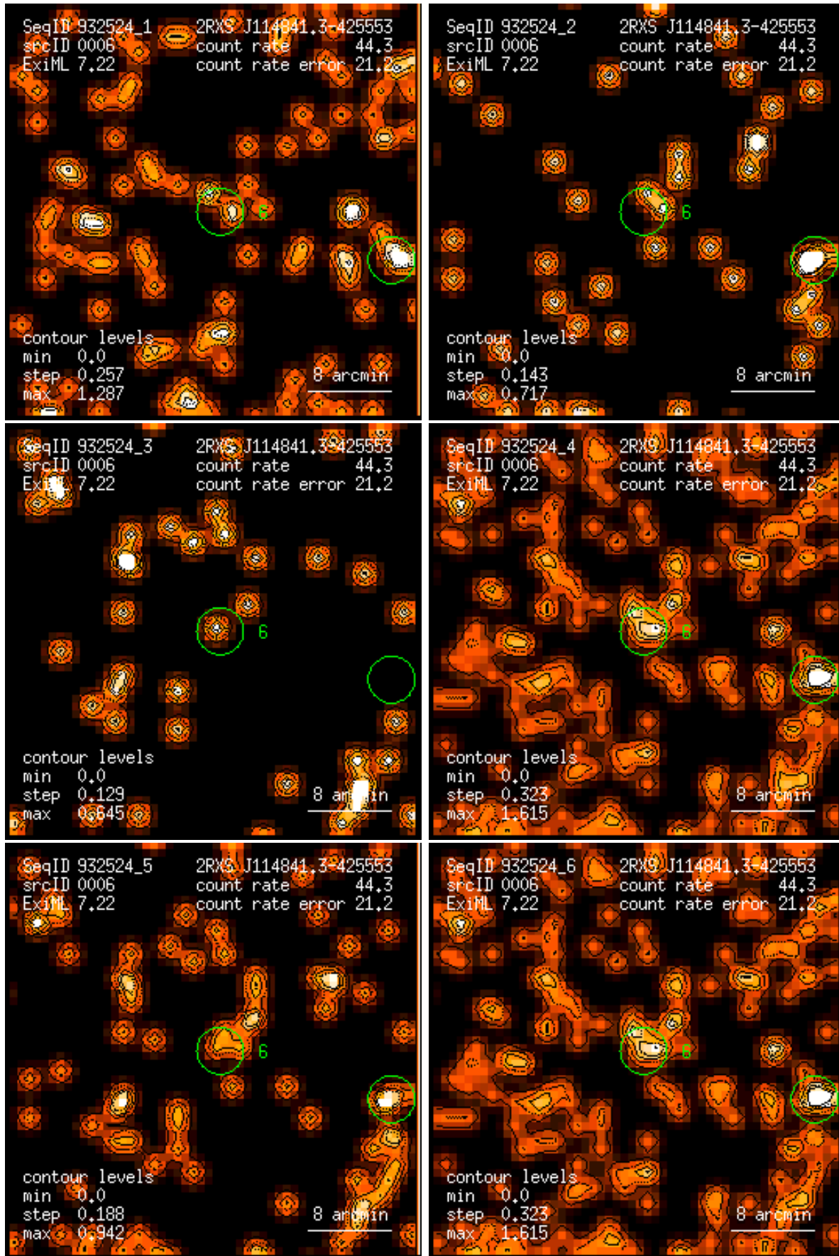
Figure 6: RASS 932524: detection 0006: band rate images, Gaussian filter: (1) PSPC channels 11 – 41, (2) 52 – 90, (3) 91 – 201, (4) 11 – 235, (5) 52 – 201, (6) 11 – 201. Broad band rates in counts/ks. Band rate contour levels in counts/ks/arcmin 2 .
