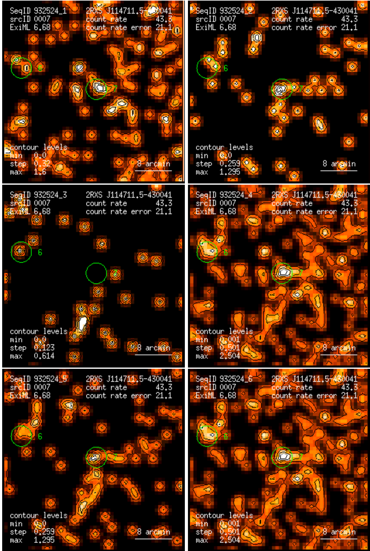
Figure 7: RASS 932524: detection 0007: band rate images, Gaussian filter: (1) PSPC channels 11 – 41, (2) 52 – 90, (3) 91 – 201, (4) 11 – 235, (5) 52 – 201, (6) 11 – 201. Broad band rates in counts/ks. Band rate contour levels in counts/ks/arcmin 2 .
