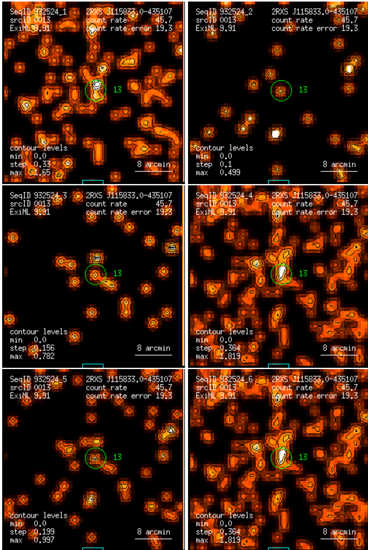
Figure 13: RASS 932524: detection 0013: band rate images, Gaussian filter: (1) PSPC channels 11 – 41, (2) 52 – 90, (3) 91 – 201, (4) 11 – 235, (5) 52 – 201, (6) 11 – 201. Broad band rates in counts/ks. Band rate contour levels in counts/ks/arcmin 2 .
