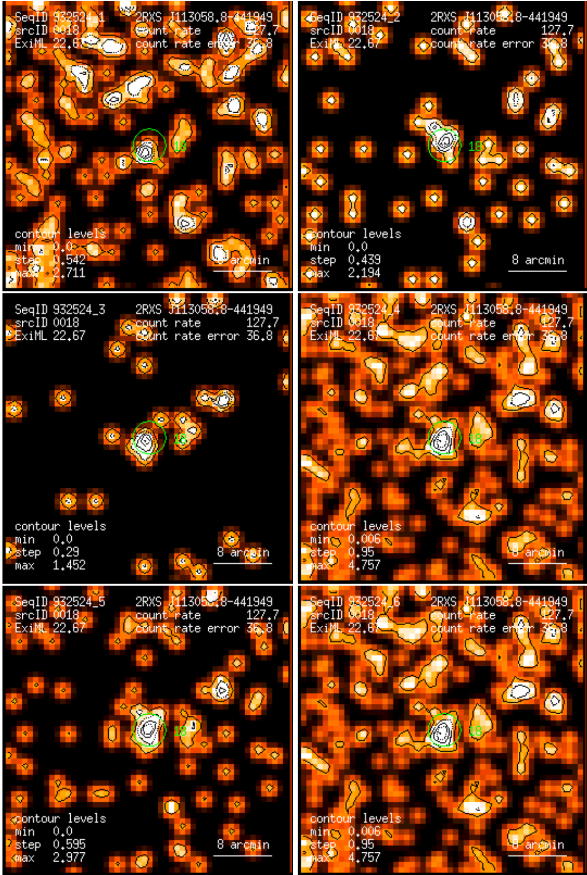
Figure 18: RASS 932524: detection 0018: band rate images, Gaussian filter: (1) PSPC channels 11 – 41, (2) 52 – 90, (3) 91 – 201, (4) 11 – 235, (5) 52 – 201, (6) 11 – 201. Broad band rates in counts/ks. Band rate contour levels in counts/ks/arcmin 2 .
