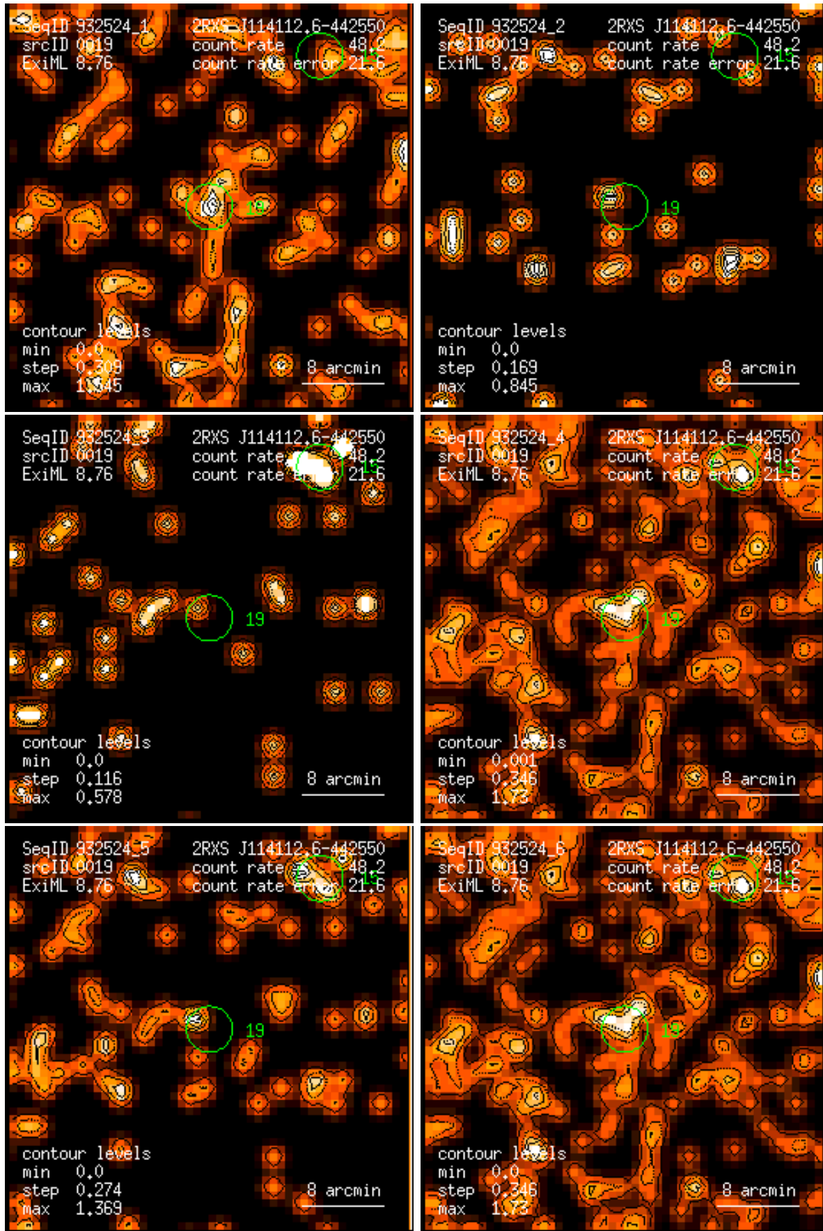
Figure 19: RASS 932524: detection 0019: band rate images, Gaussian filter: (1) PSPC channels 11 – 41, (2) 52 – 90, (3) 91 – 201, (4) 11 – 235, (5) 52 – 201, (6) 11 – 201. Broad band rates in counts/ks. Band rate contour levels in counts/ks/arcmin 2 .
